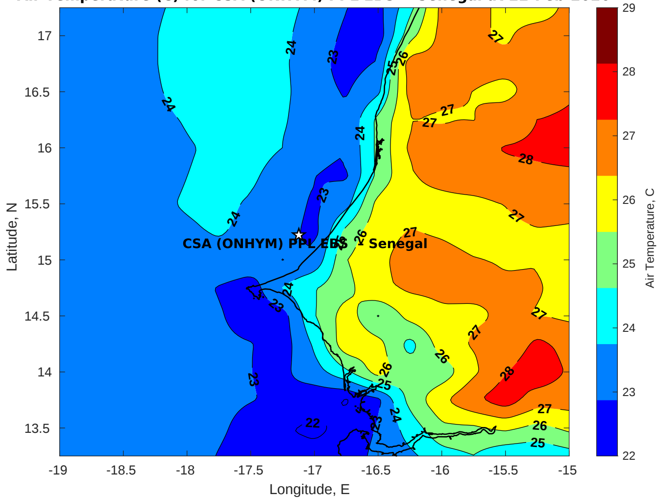
Air Temperature (C) for CSA (ONHYM) PPL EBS - Senegal at 22-Feb-2026
