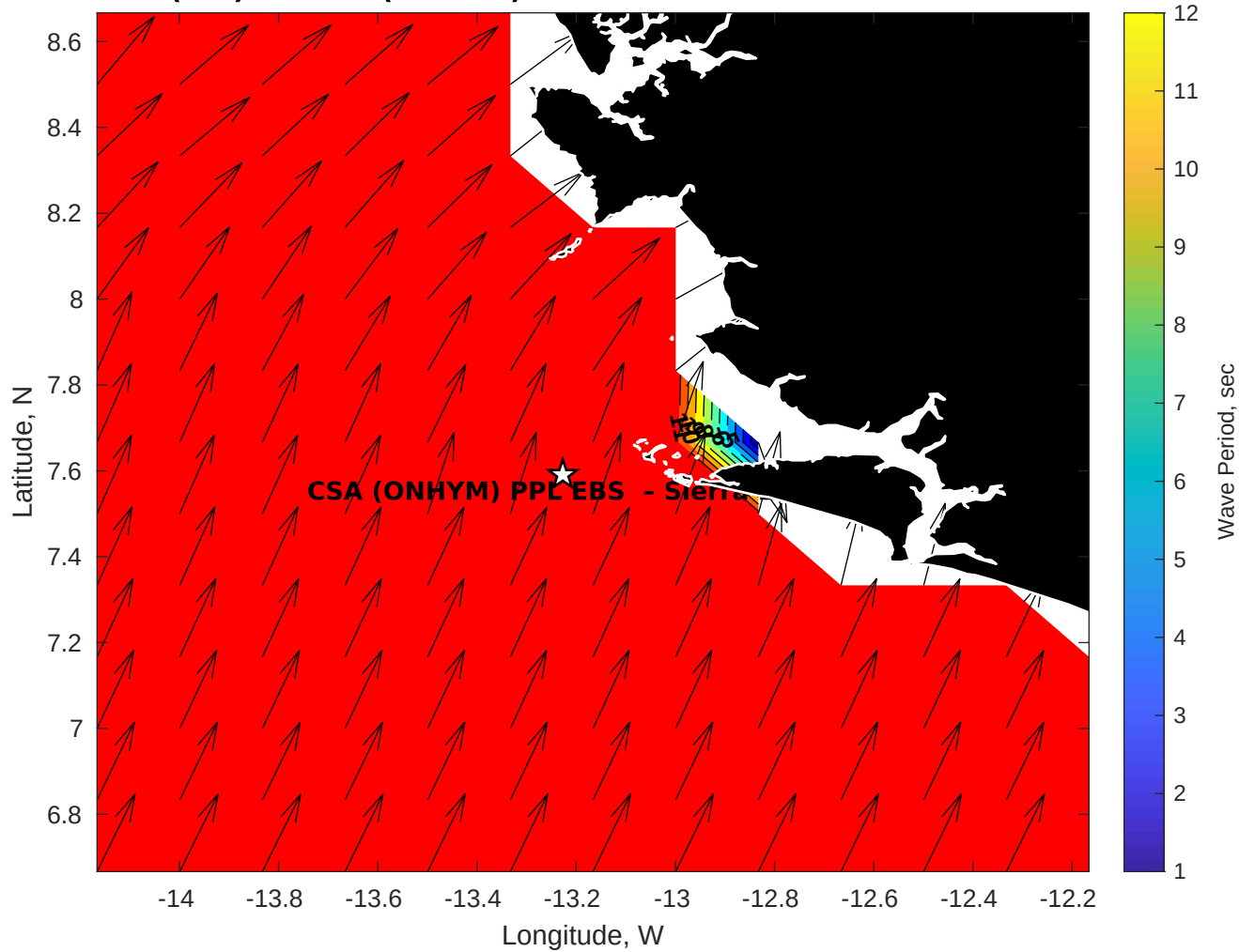
GFS Wave Period (sec) for CSA (ONHYM) PPL EBS - Sierra Leone at 22-Feb-2026 09:00:00
