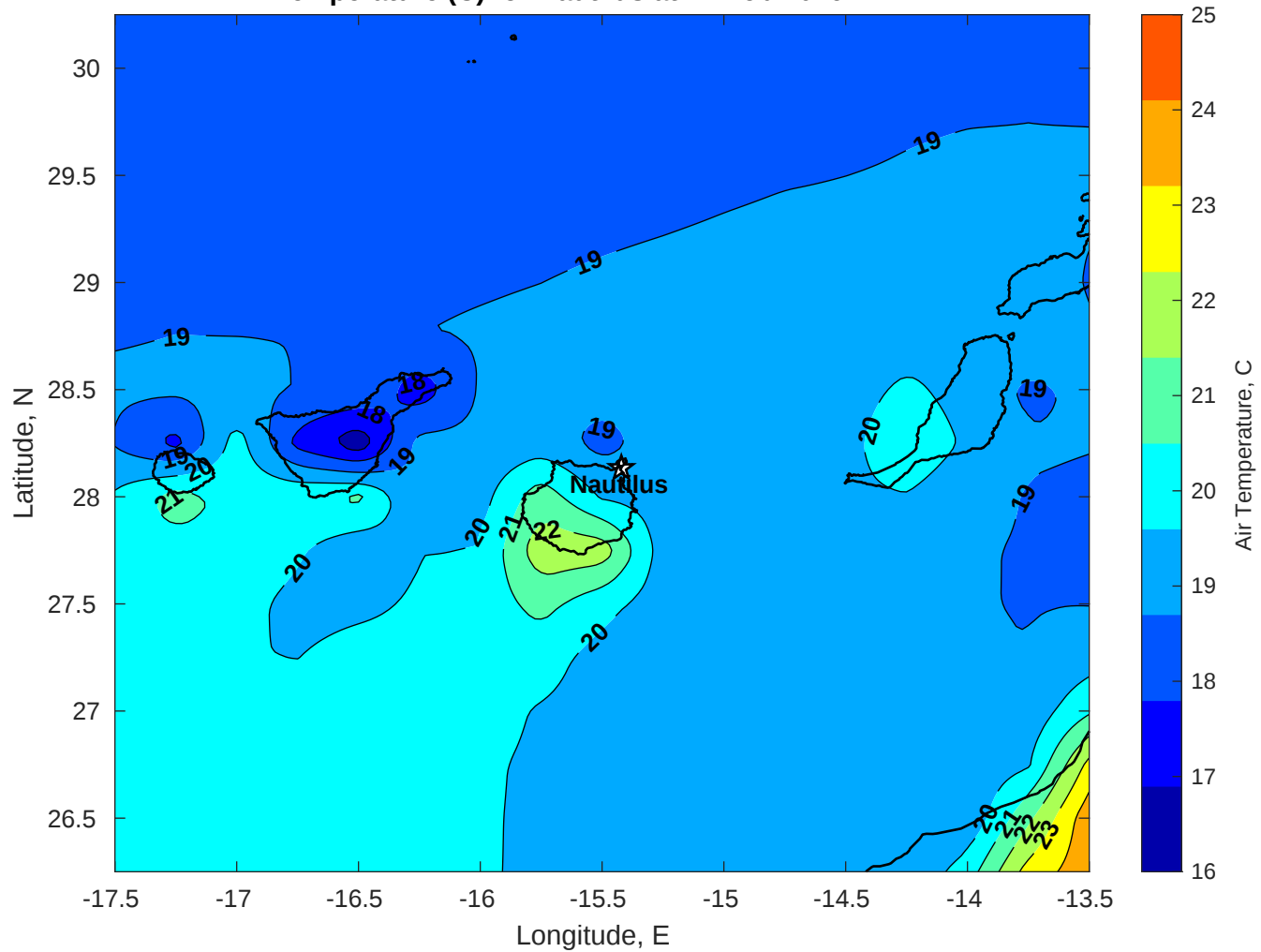
Air Temperature (C) for Nautilus at 22-Feb-2026
