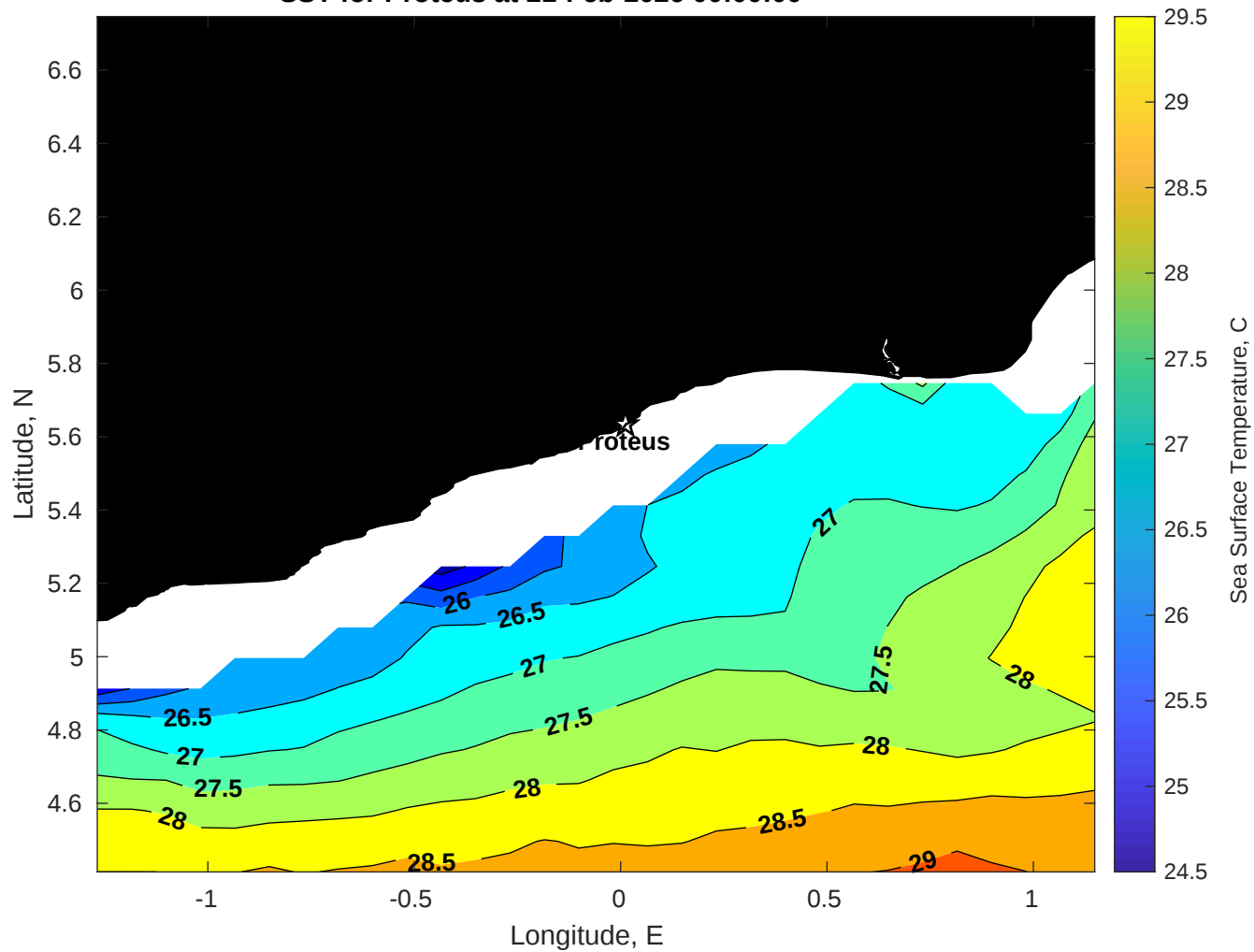
SST for Proteus at 21-Feb-2026 00:00:00
