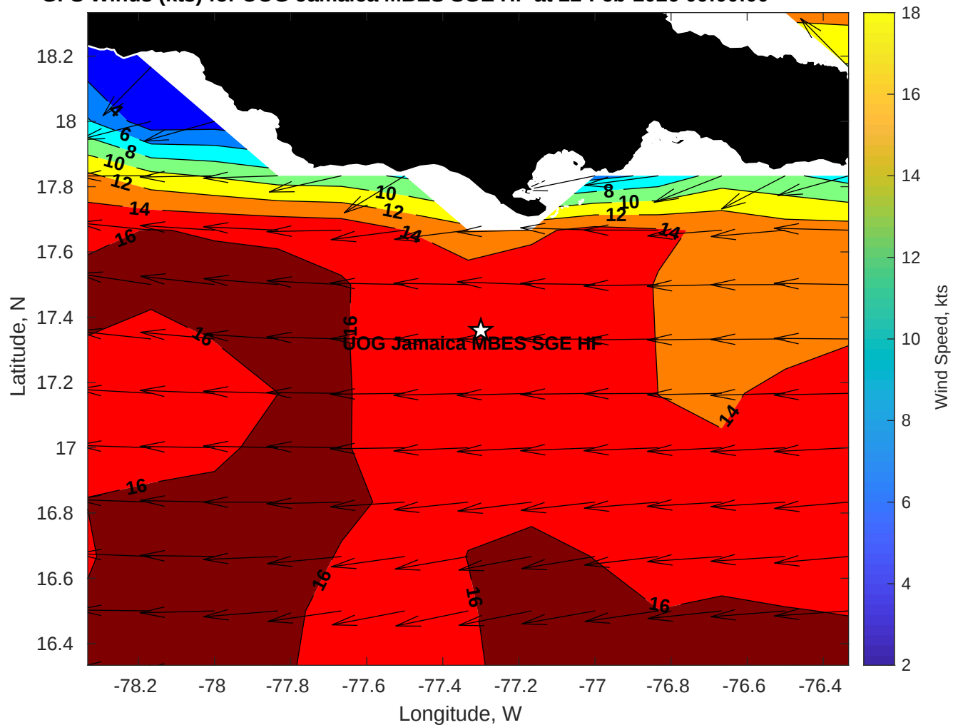
GFS Winds (kts) for UOG Jamaica MBES SGE HF at 22-Feb-2026 09:00:00
