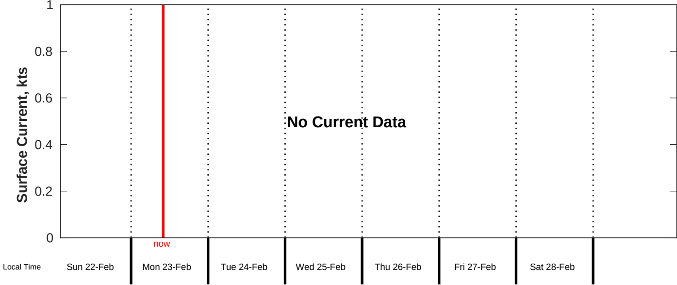
Surface Current Forecast for CSA (ONHYM) PPL EBS - Cote d'Ivoire from 22-Feb-2026 00:00:00 to 02-Mar-2026 00:00:00
