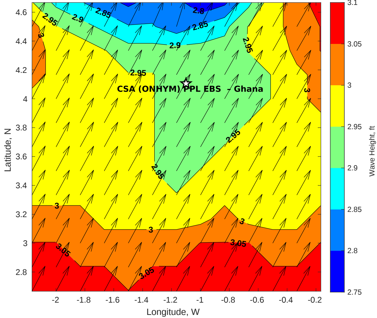
GFS Wave Height (ft) for CSA (ONHYM) PPL EBS - Ghana at 23-Feb-2026 09:00:00
