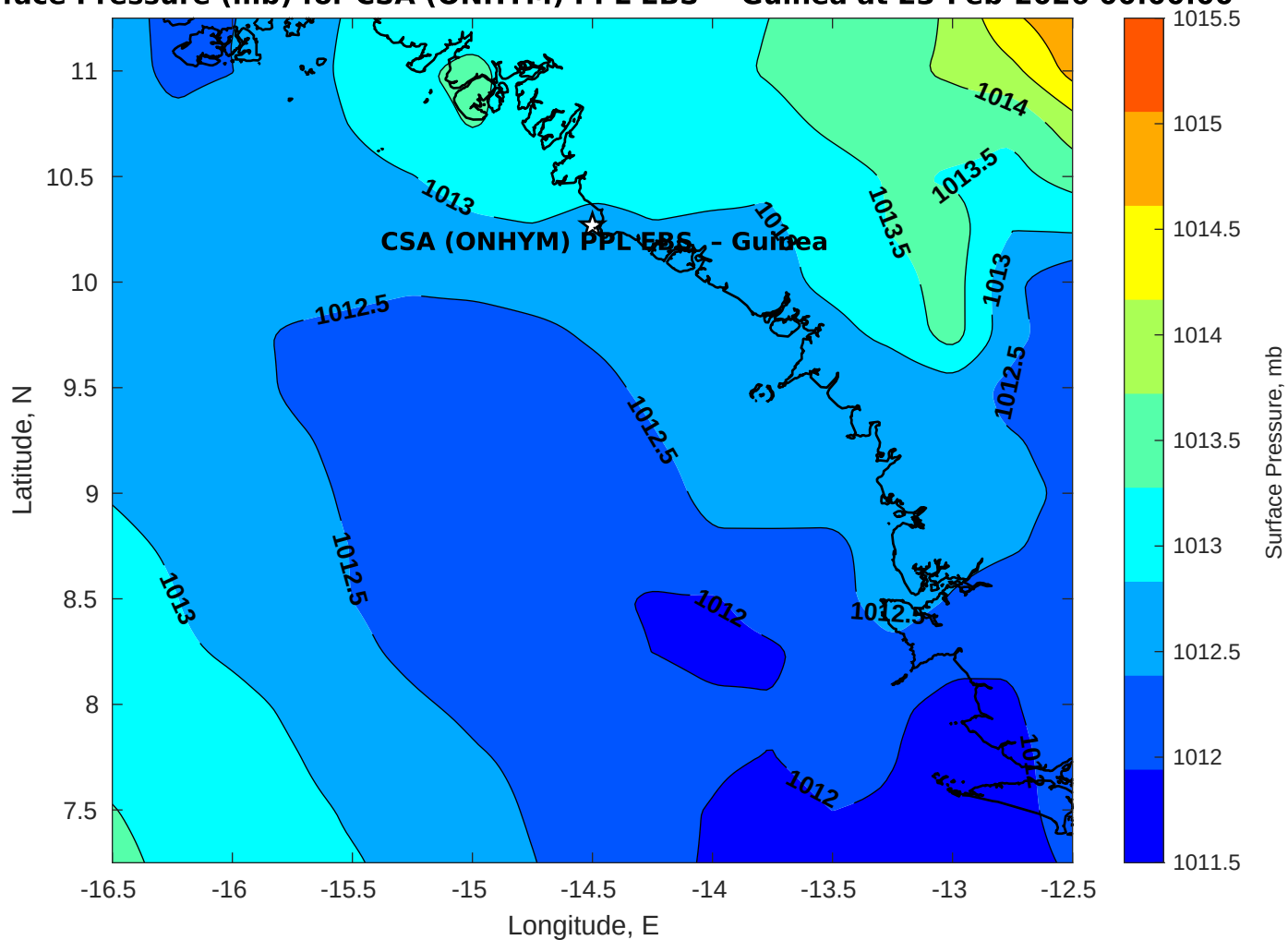
Surface Pressure (mb) for CSA (ONHYM) PPL EBS - Guinea at 23-Feb-2026 00:00:00
