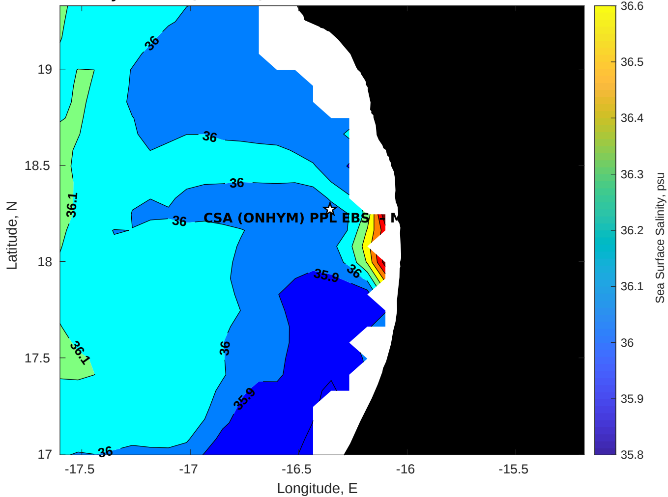
Surface Salinity for CSA (ONHYM) PPL EBS - Mauritania at 22-Feb-2026 00:00:00
