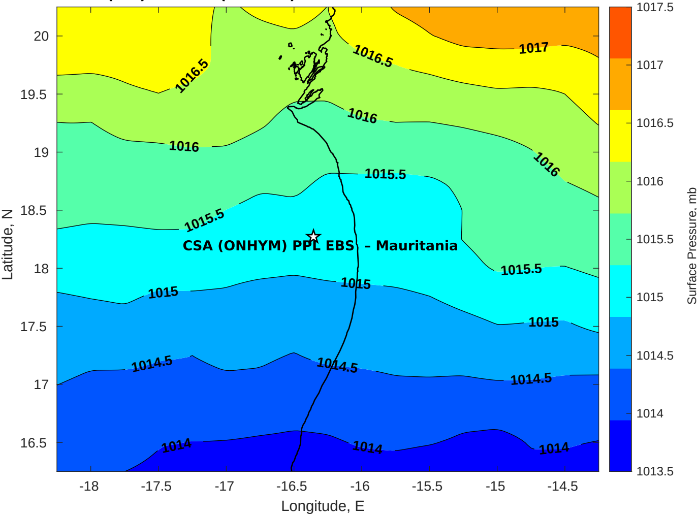
Surface Pressure (mb) for CSA (ONHYM) PPL EBS - Mauritania at 23-Feb-2026 00:00:00
