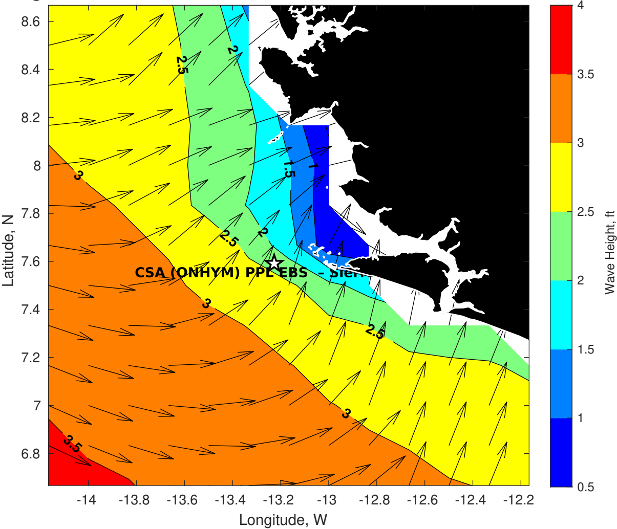
GFS Wave Height (ft) for CSA (ONHYM) PPL EBS - Sierra Leone at 23-Feb-2026 09:00:00
