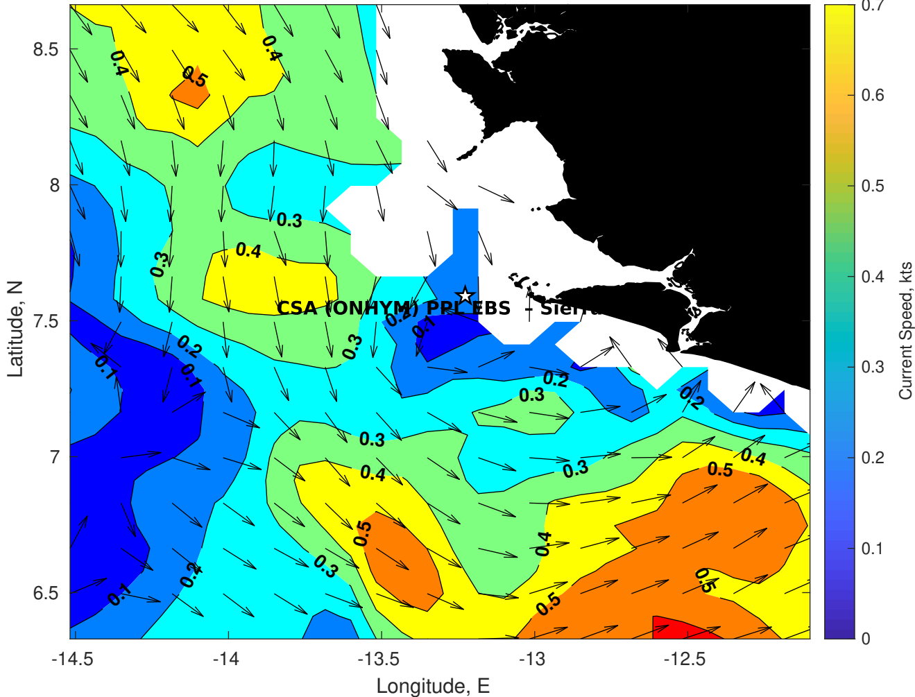
Surface Currents for CSA (ONHYM) PPL EBS - Sierra Leone at 22-Feb-2026 00:00:00
