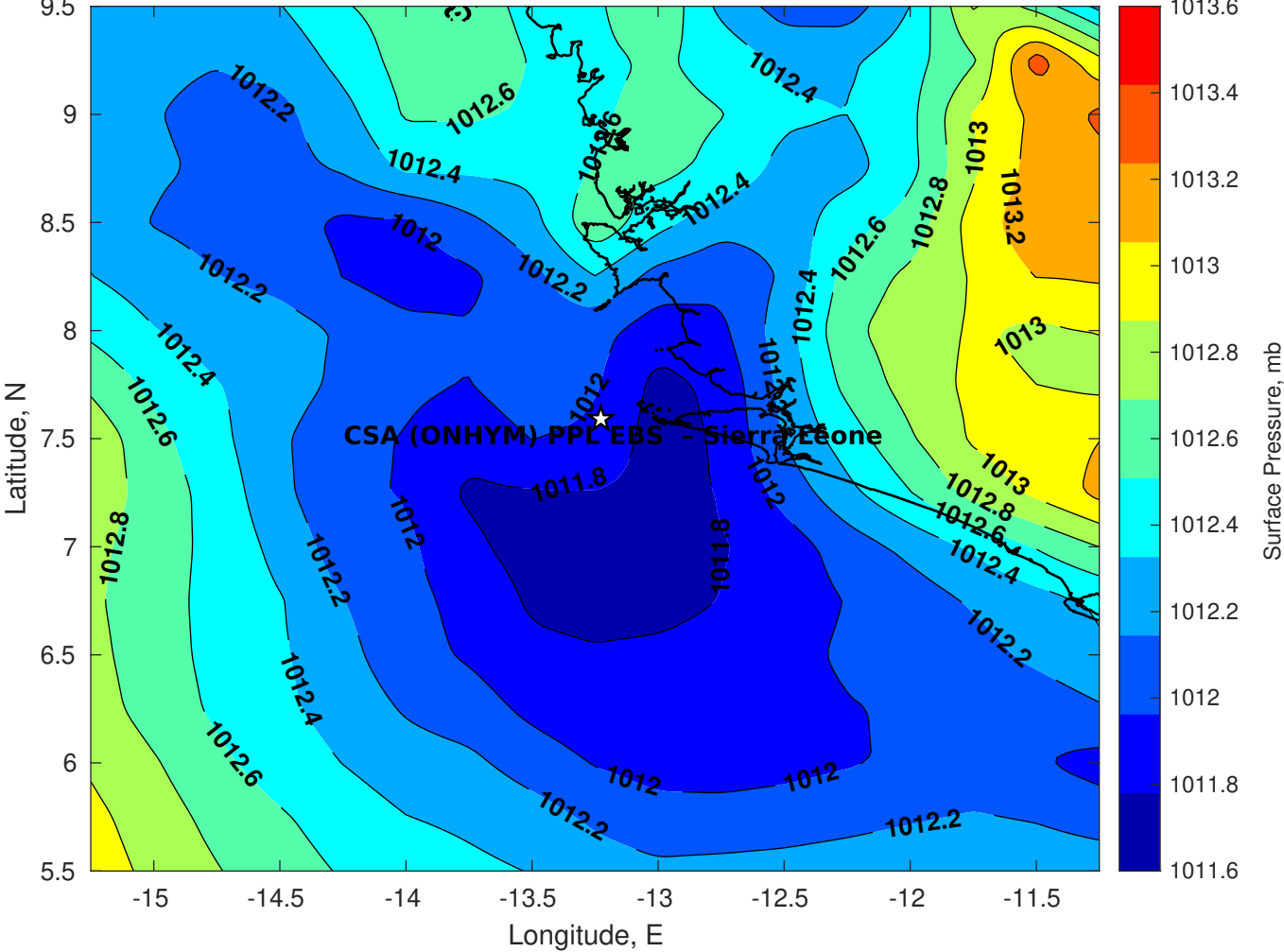
Surface Pressure (mb) for CSA (ONHYM) PPL EBS - Sierra Leone at 23-Feb-2026 00:00:00
