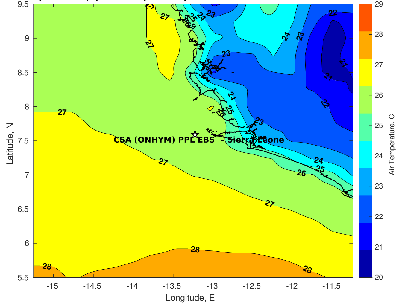
Air Temperature (C) for CSA (ONHYM) PPL EBS - Sierra Leone at 23-Feb-2026
