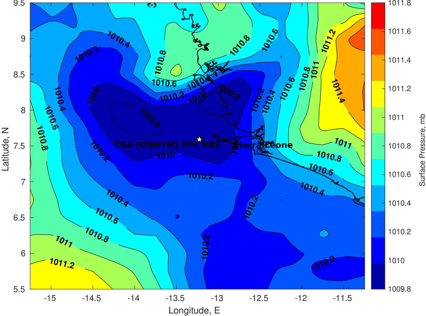
Surface Pressure (mb) for CSA (ONHYM) PPL EBS - Sierra Leone at 24-Feb-2026 00:00:00
