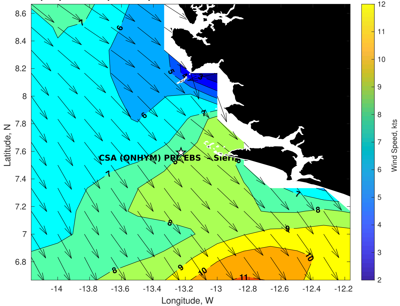
GFS Winds (kts) for CSA (ONHYM) PPL EBS - Sierra Leone at 23-Feb-2026 09:00:00
