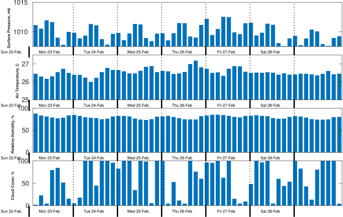
Met Forecast for CSA (ONHYM) PPL EBS - Sierra Leone from 23-Feb-2026 00:00:00 to 02-Mar-2026 00:00:00
