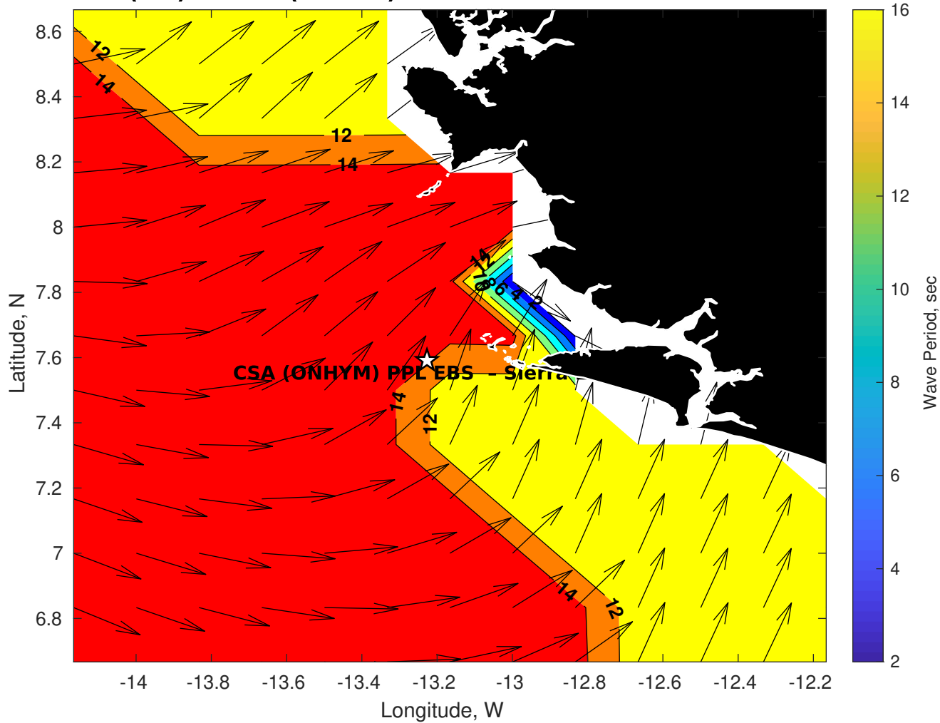
GFS Wave Period (sec) for CSA (ONHYM) PPL EBS - Sierra Leone at 23-Feb-2026 09:00:00
