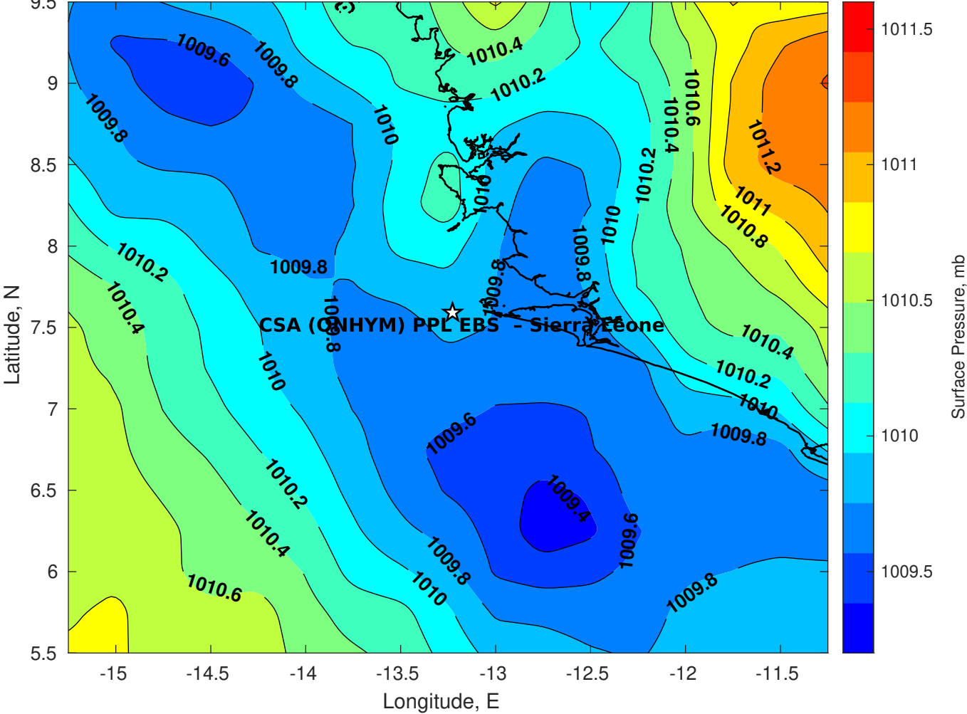
Surface Pressure (mb) for CSA (ONHYM) PPL EBS - Sierra Leone at 25-Feb-2026 00:00:00
