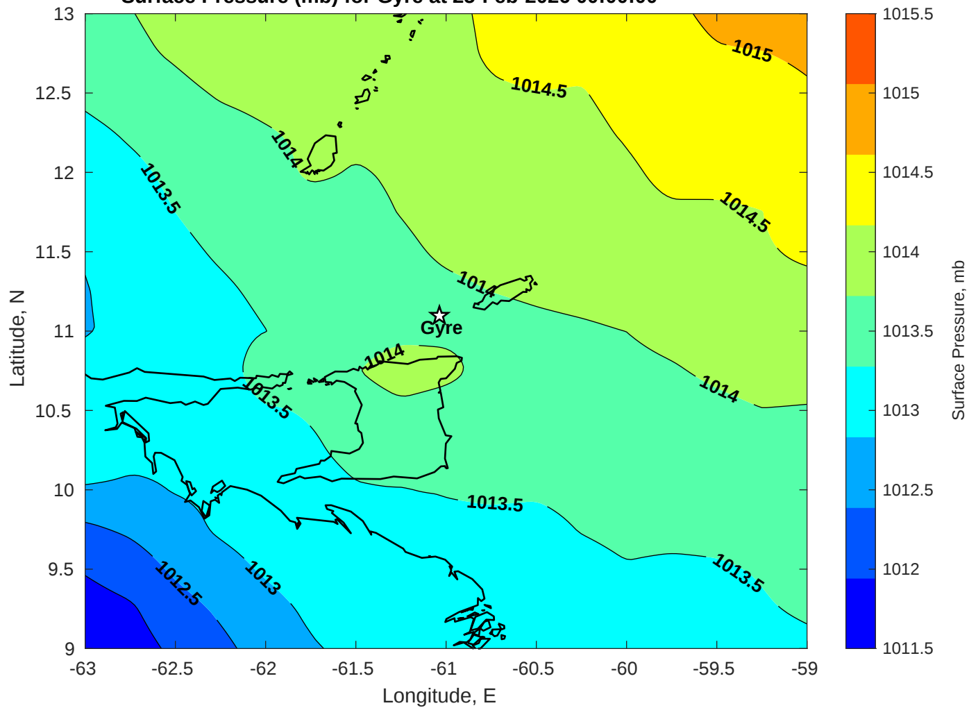
Surface Pressure (mb) for Gyre at 25-Feb-2026 00:00:00
