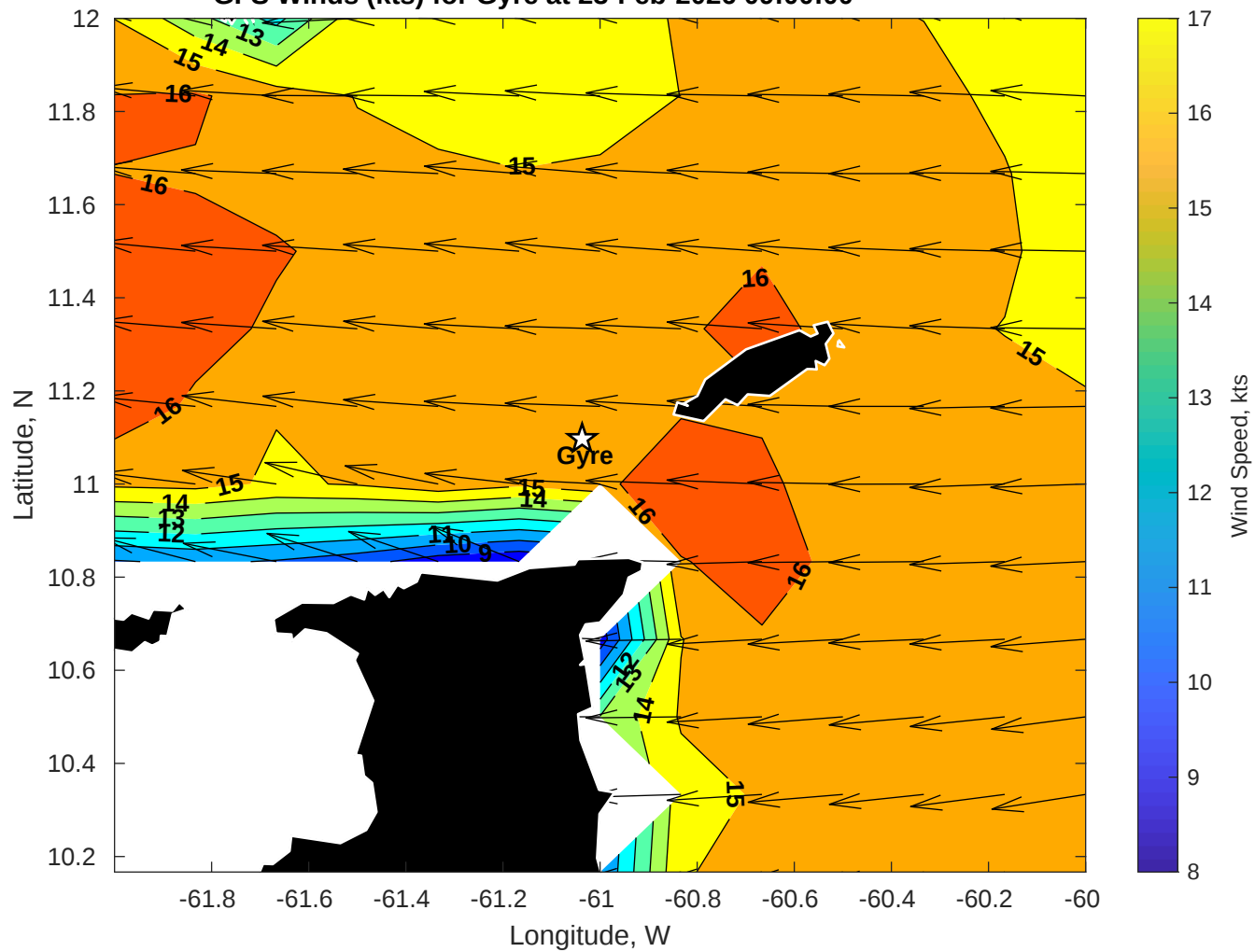
GFS Winds (kts) for Gyre at 23-Feb-2026 09:00:00
