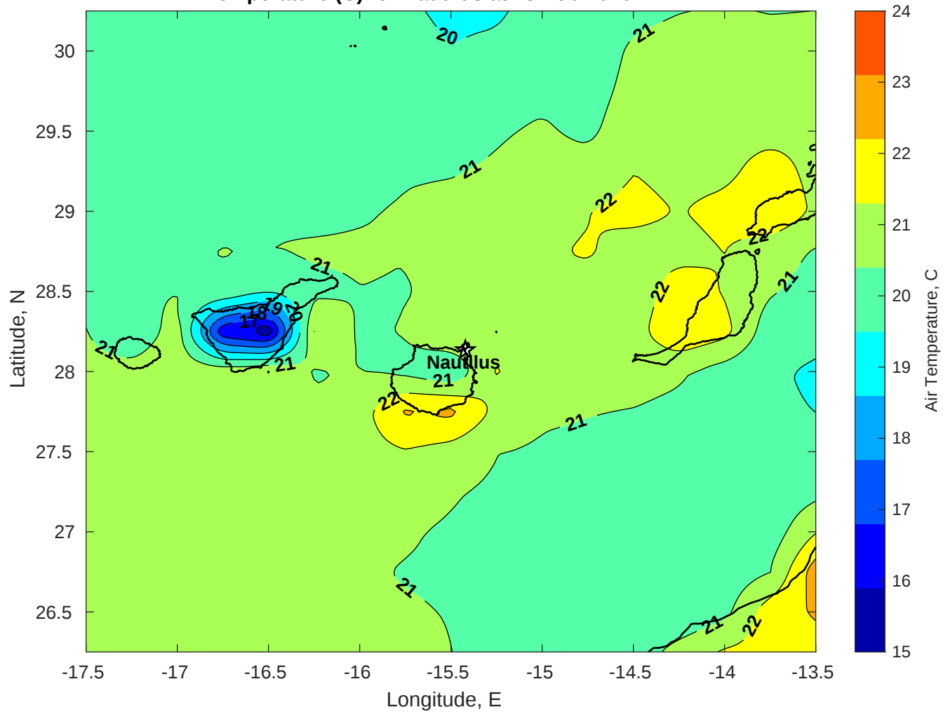
Air Temperature (C) for Nautilus at 23-Feb-2026
