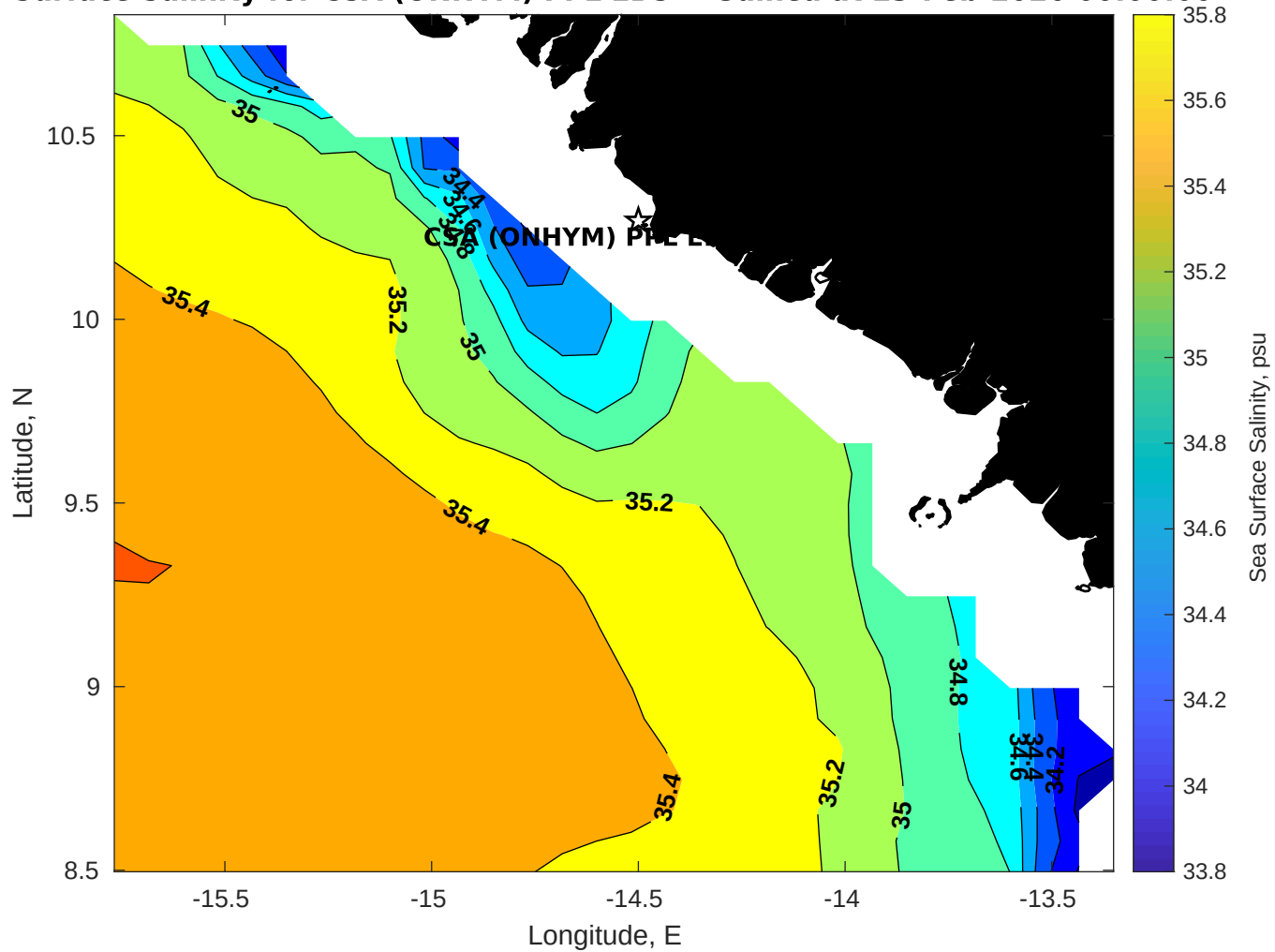
Surface Salinity for CSA (ONHYM) PPL EBS - Guinea at 23-Feb-2026 00:00:00
