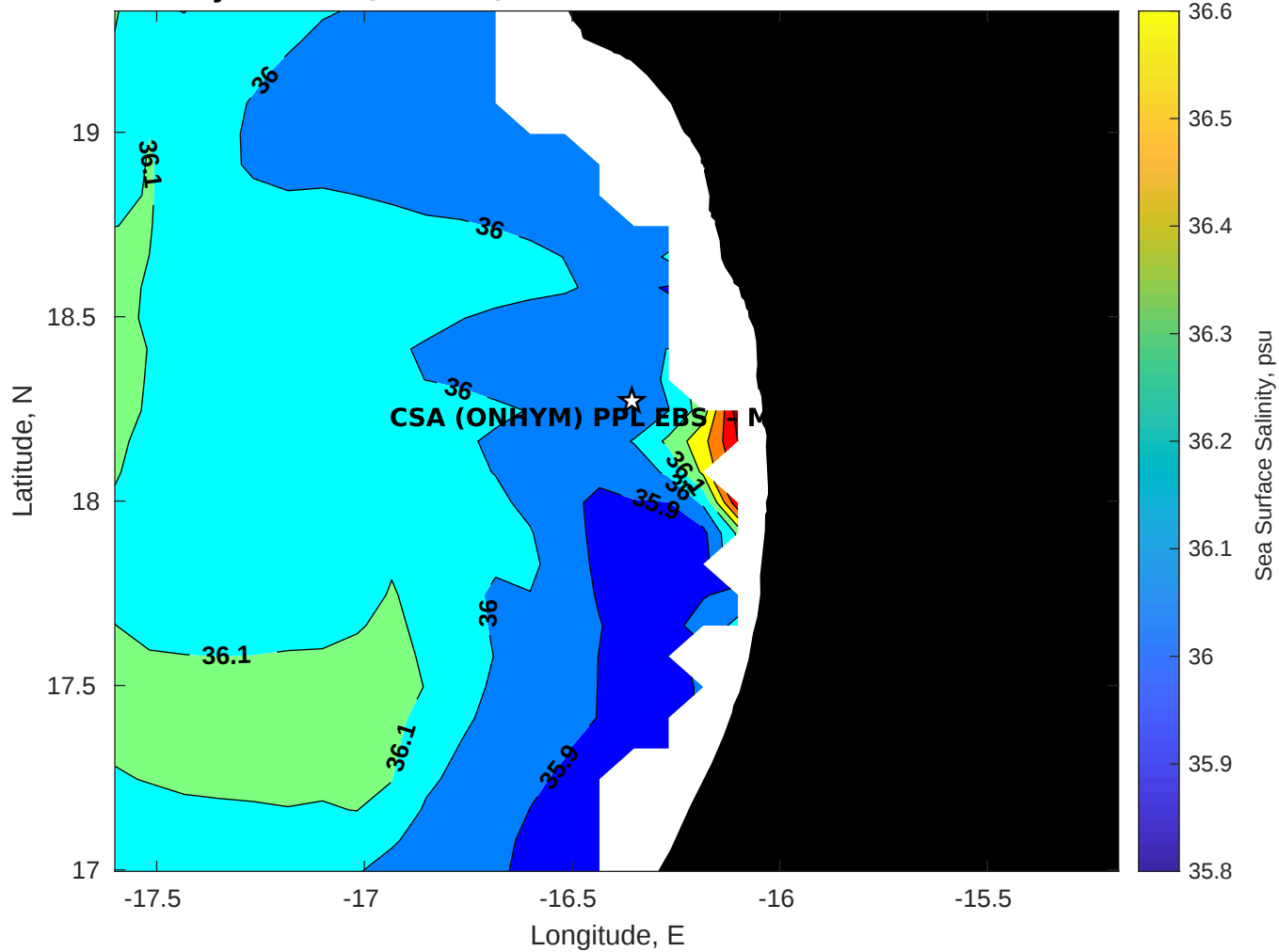
Surface Salinity for CSA (ONHYM) PPL EBS - Mauritania at 23-Feb-2026 00:00:00
