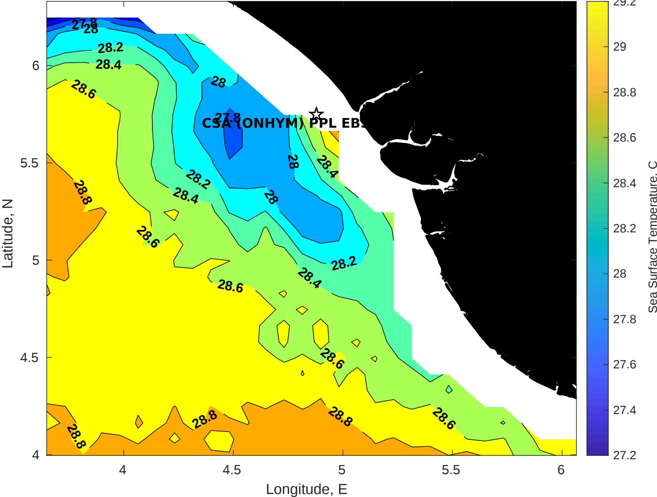
SST for CSA (ONHYM) PPL EBS - Nigeria at 23-Feb-2026 00:00:00
