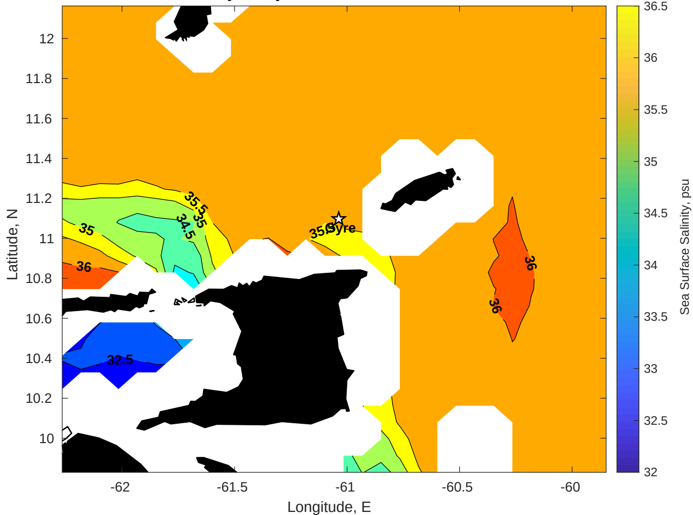
Surface Salinity for Gyre at 23-Feb-2026 00:00:00
