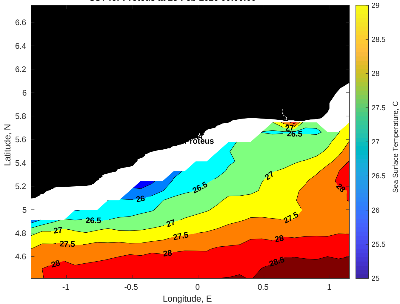
SST for Proteus at 23-Feb-2026 00:00:00
