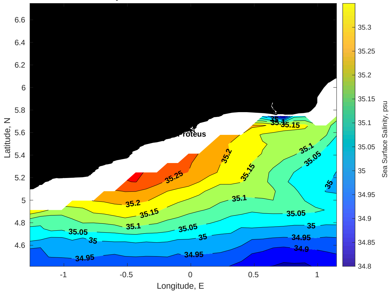
Surface Salinity for Proteus at 23-Feb-2026 00:00:00
