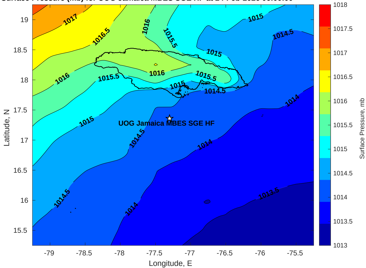
Surface Pressure (mb) for UOG Jamaica MBES SGE HF at 24-Feb-2026 06:00:00
