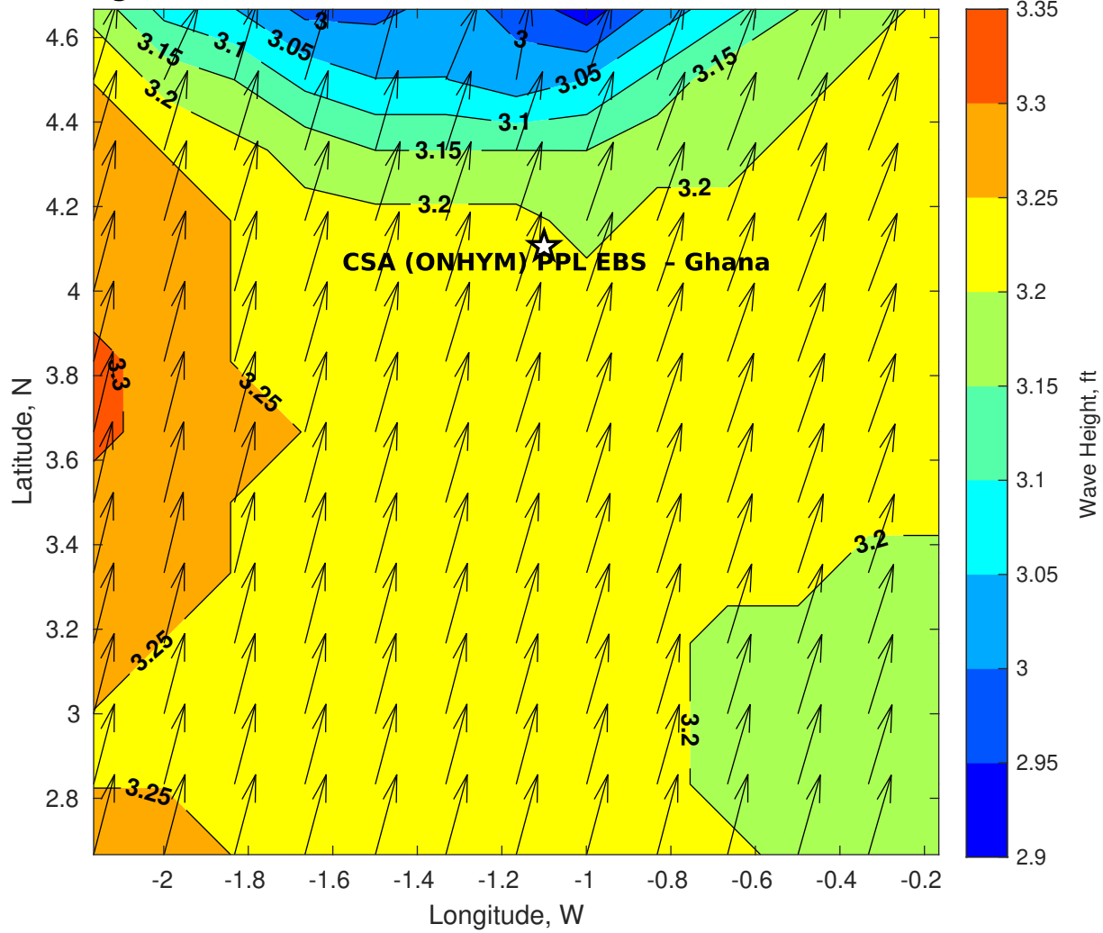
GFS Wave Height (ft) for CSA (ONHYM) PPL EBS - Ghana at 24-Feb-2026 09:00:00
