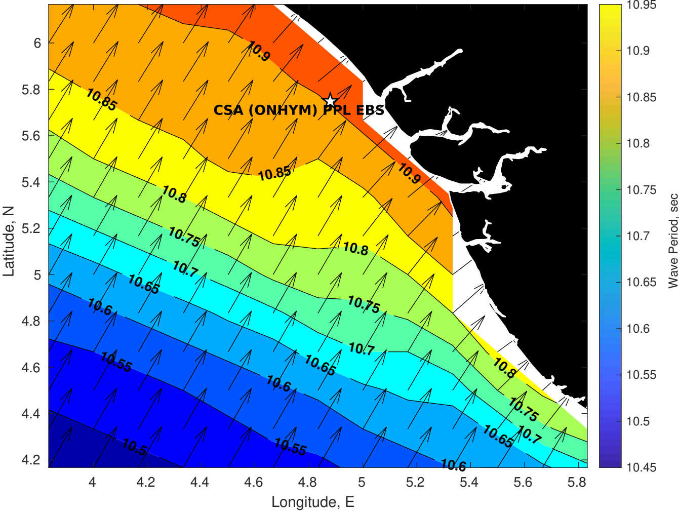
GFS Wave Period (sec) for CSA (ONHYM) PPL EBS - Nigeria at 24-Feb-2026 09:00:00
