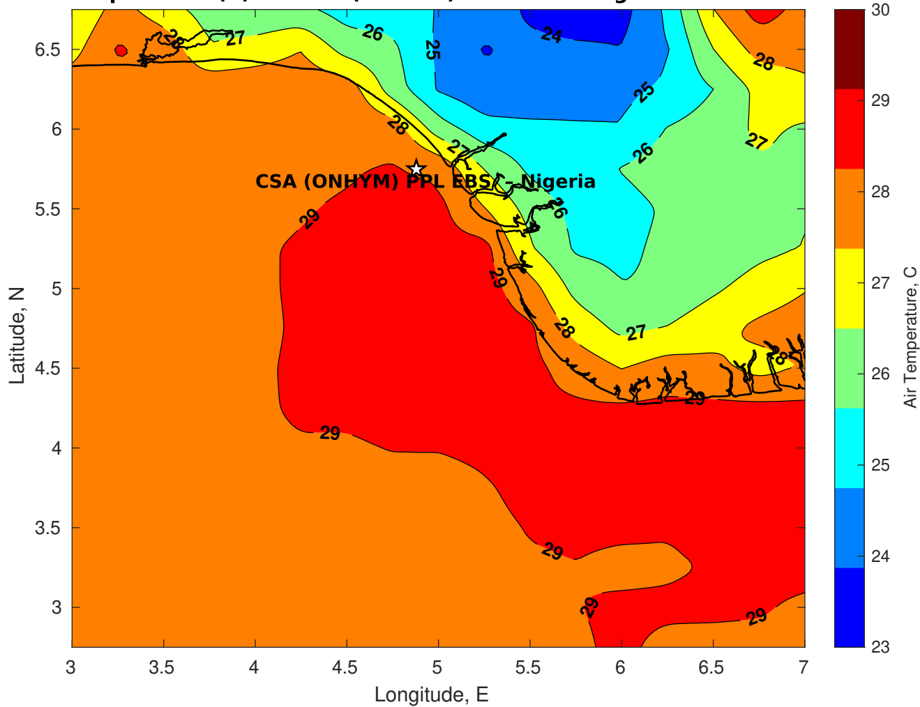
Air Temperature (C) for CSA (ONHYM) PPL EBS - Nigeria at 24-Feb-2026
