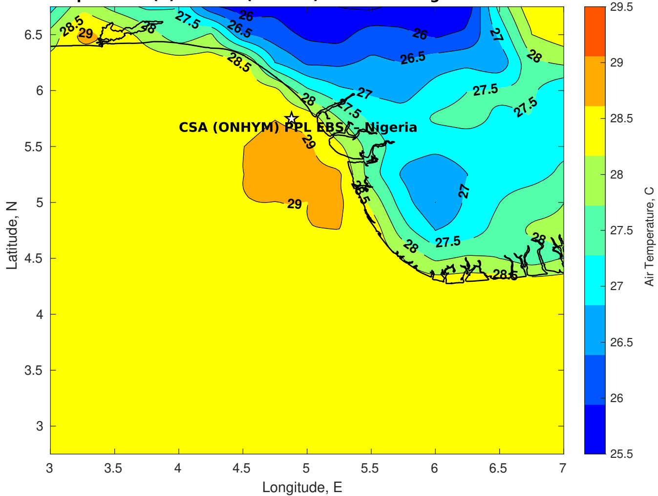
Air Temperature (C) for CSA (ONHYM) PPL EBS - Nigeria at 24-Feb-2026
