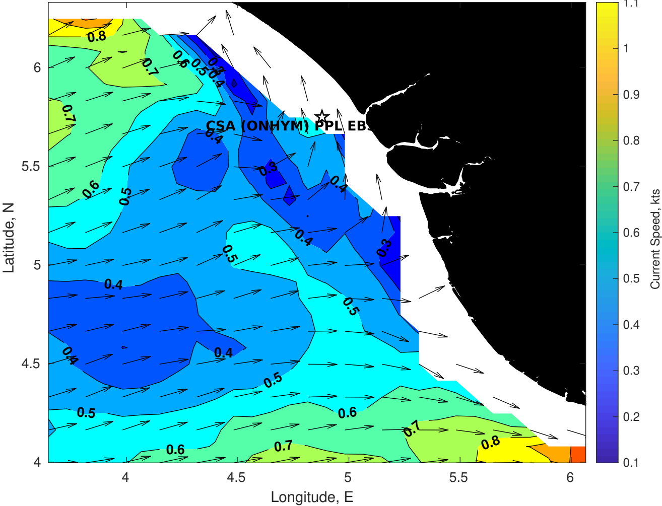
Surface Currents for CSA (ONHYM) PPL EBS - Nigeria at 23-Feb-2026 00:00:00
