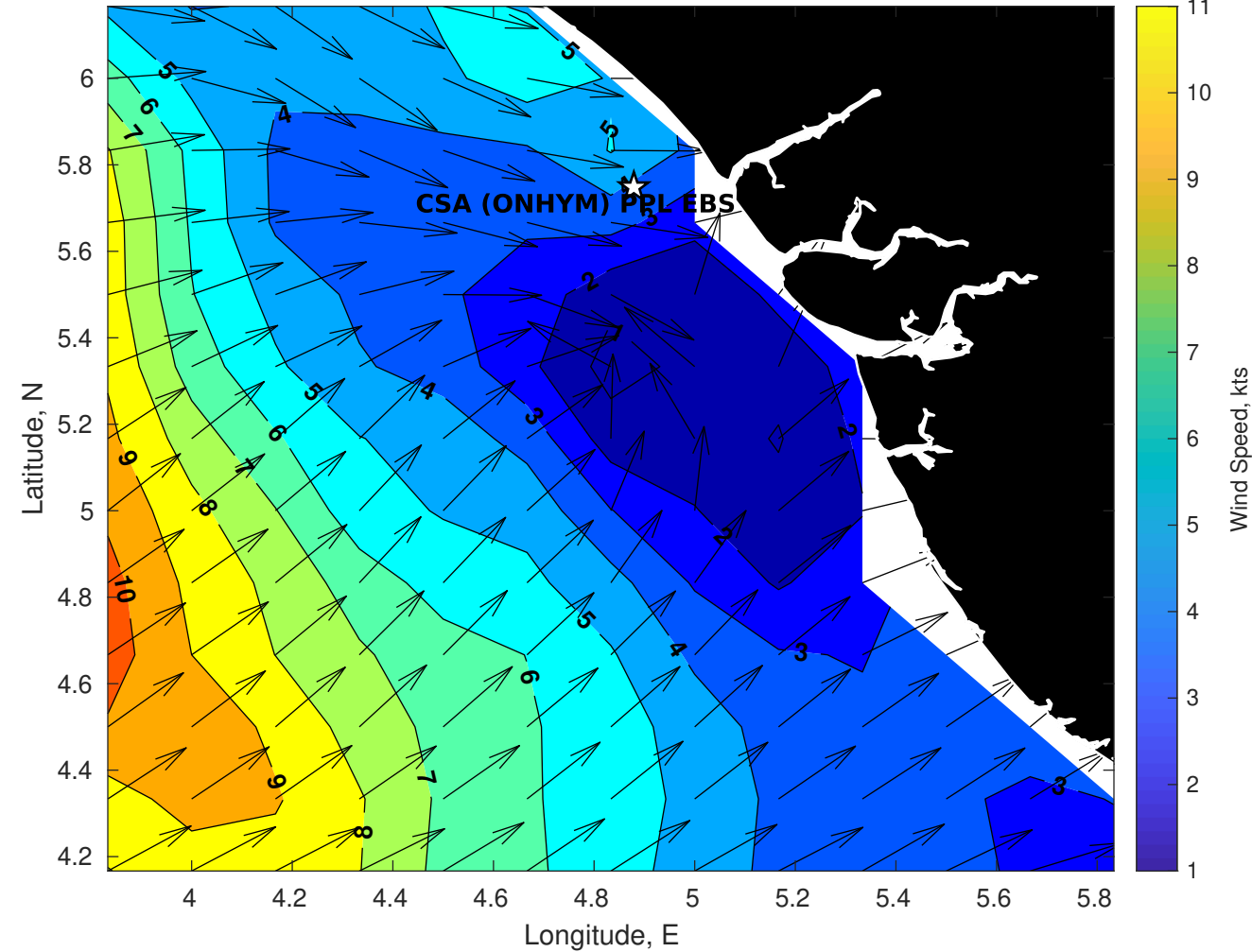
GFS Winds (kts) for CSA (ONHYM) PPL EBS - Nigeria at 24-Feb-2026 09:00:00
