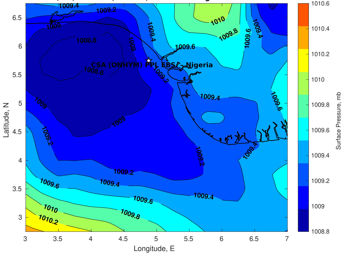
Surface Pressure (mb) for CSA (ONHYM) PPL EBS - Nigeria at 26-Feb-2026 00:00:00
