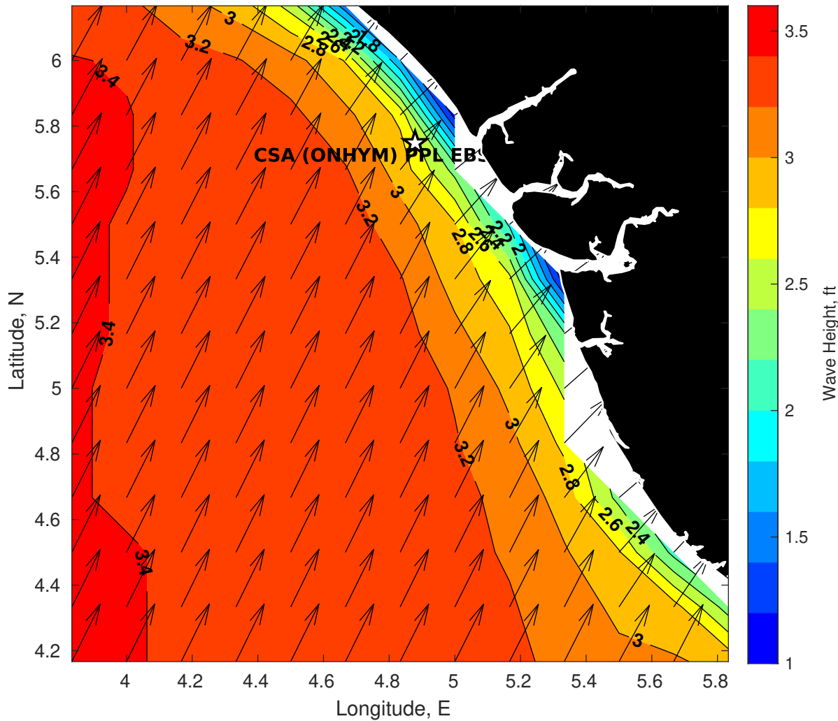
GFS Wave Height (ft) for CSA (ONHYM) PPL EBS - Nigeria at 24-Feb-2026 09:00:00
