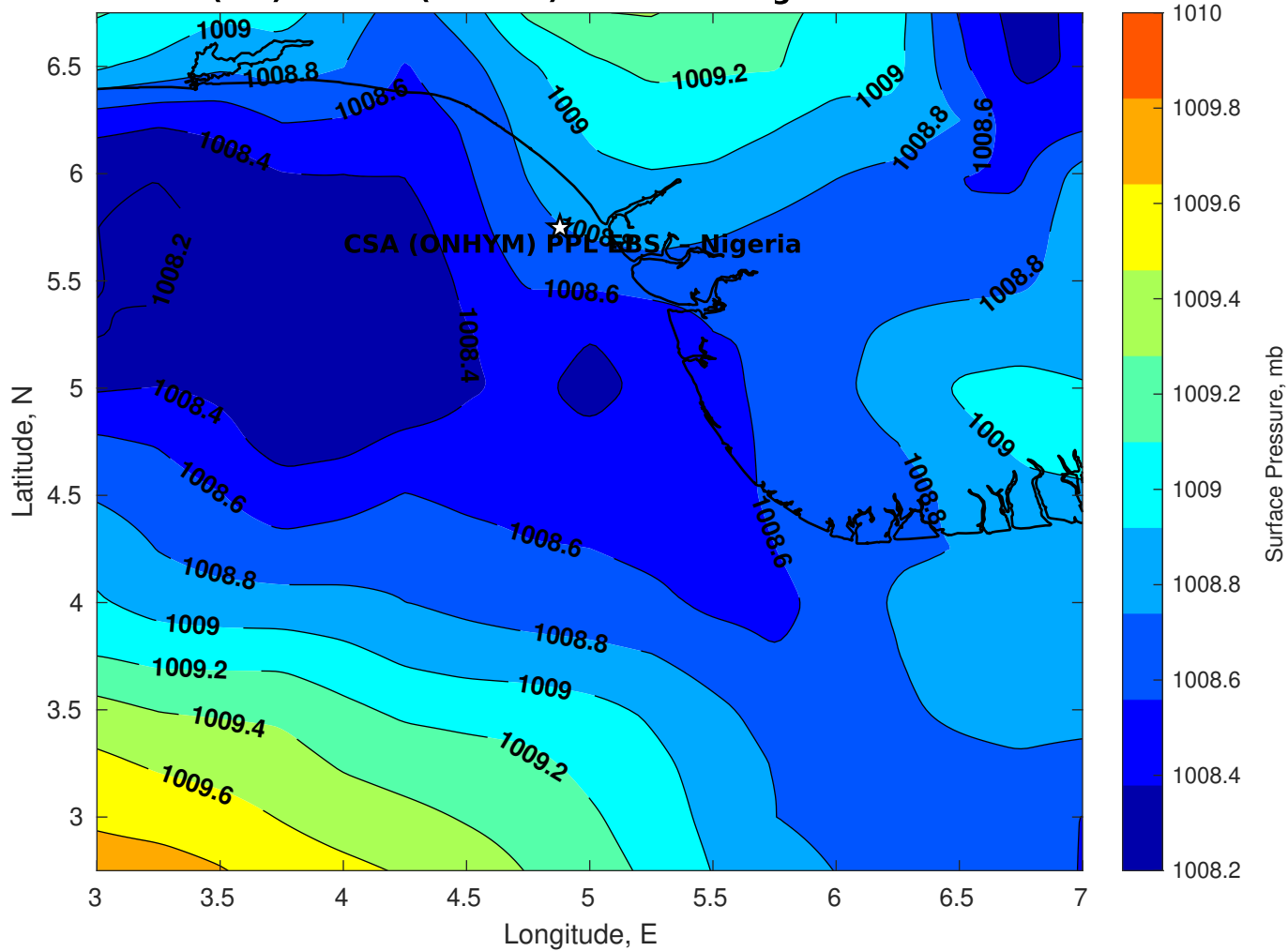
Surface Pressure (mb) for CSA (ONHYM) PPL EBS - Nigeria at 25-Feb-2026 00:00:00
