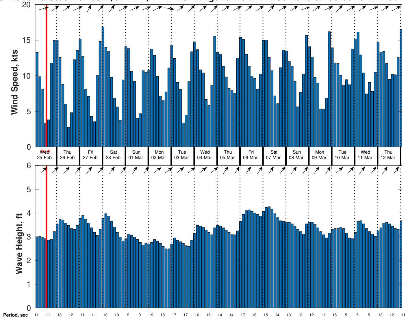
Wind & Wave Forecast for CSA (ONHYM) PPL EBS - Nigeria from 24-Feb-2026 02:00:00 to 12-Mar-2026 02:00:00
