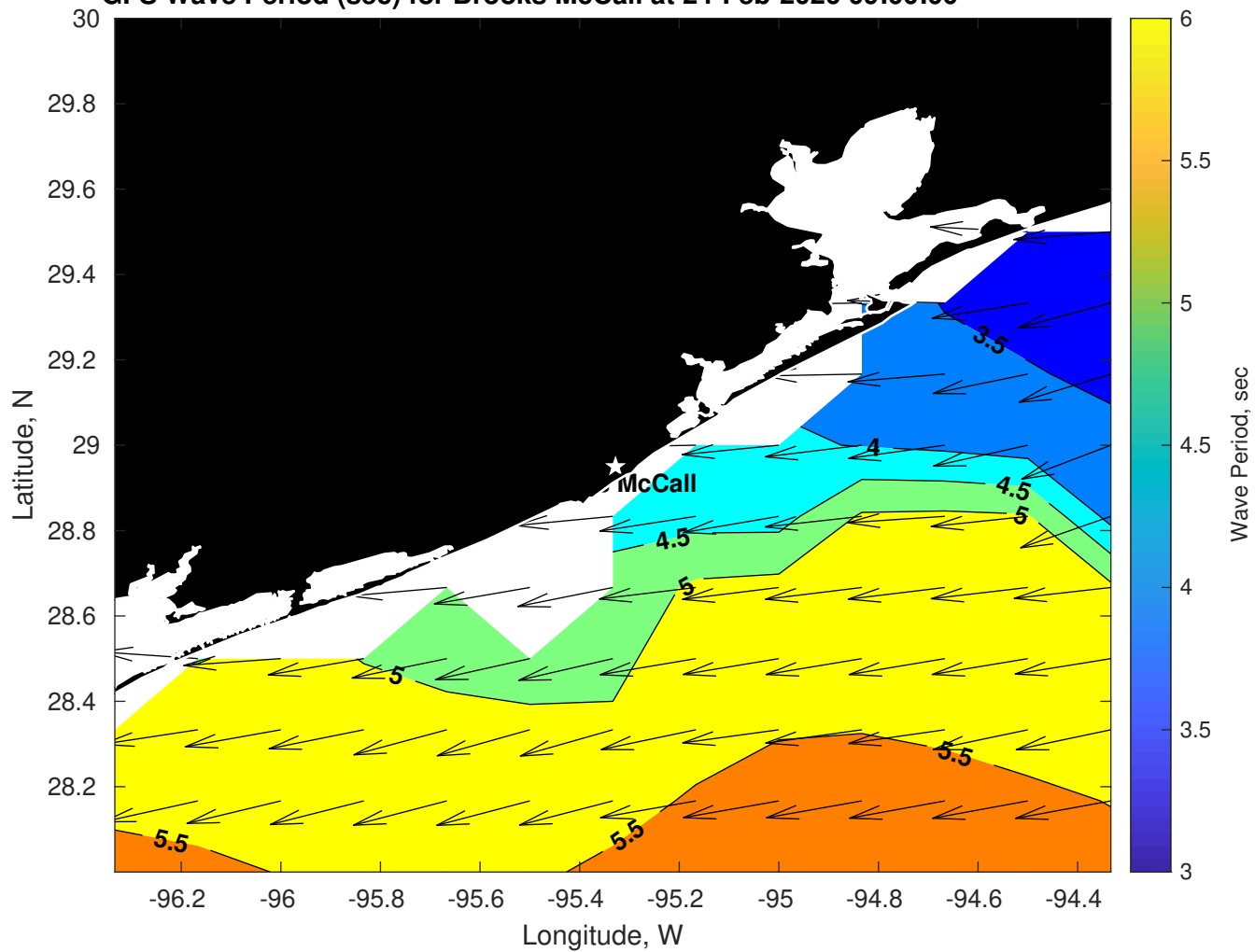
GFS Wave Period (sec) for Brooks McCall at 24-Feb-2026 09:00:00
