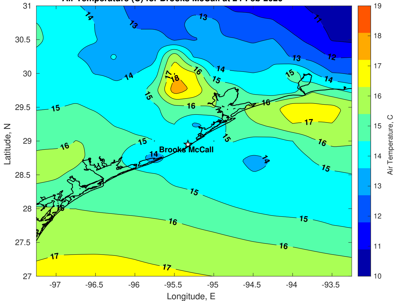
Air Temperature (C) for Brooks McCall at 24-Feb-2026
