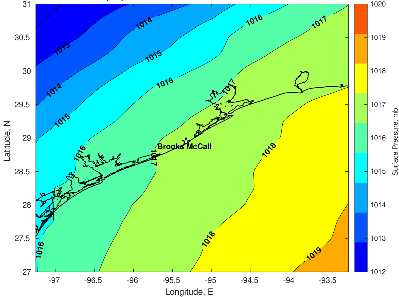
Surface Pressure (mb) for Brooks McCall at 25-Feb-2026 00:00:00
