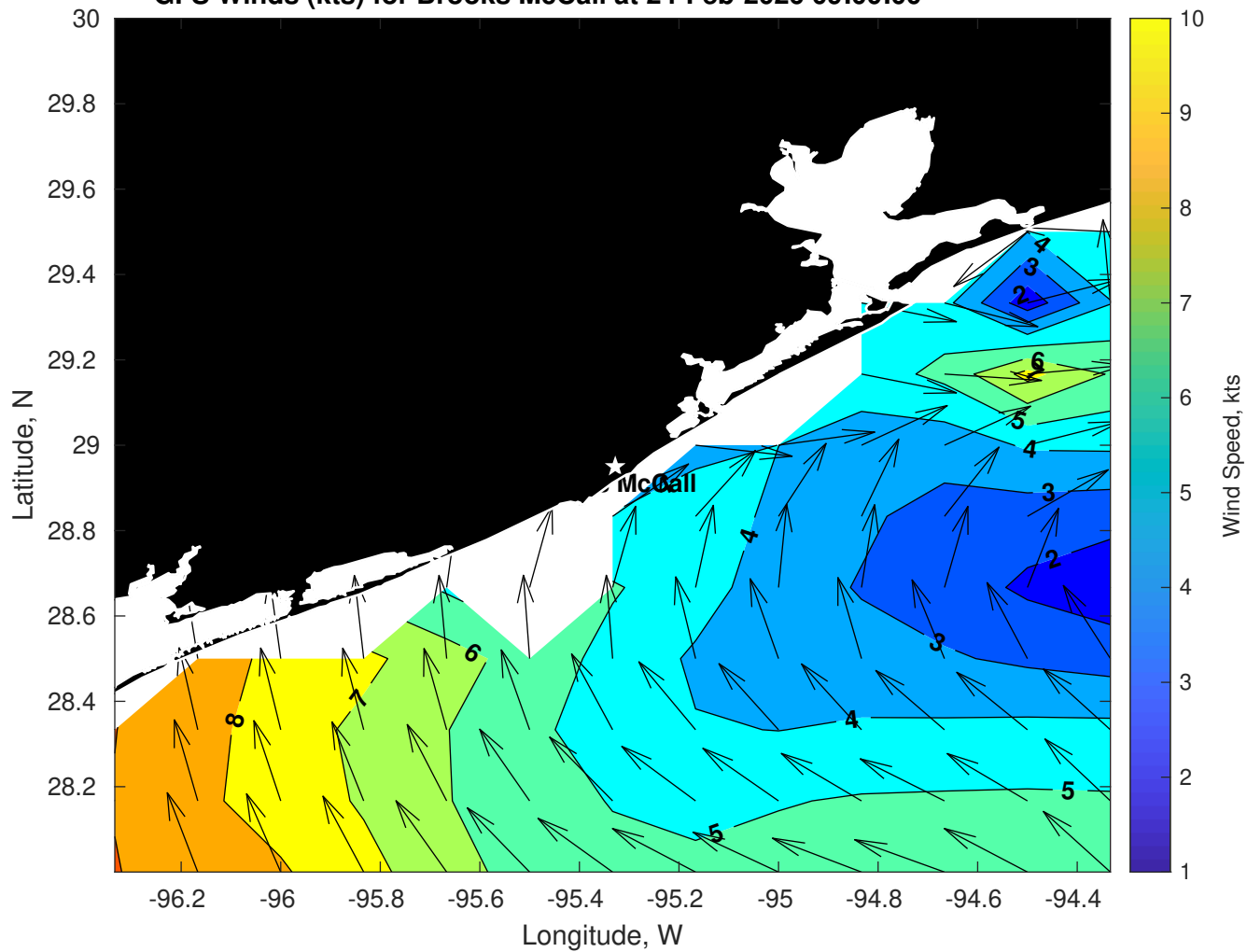
GFS Winds (kts) for Brooks McCall at 24-Feb-2026 09:00:00
