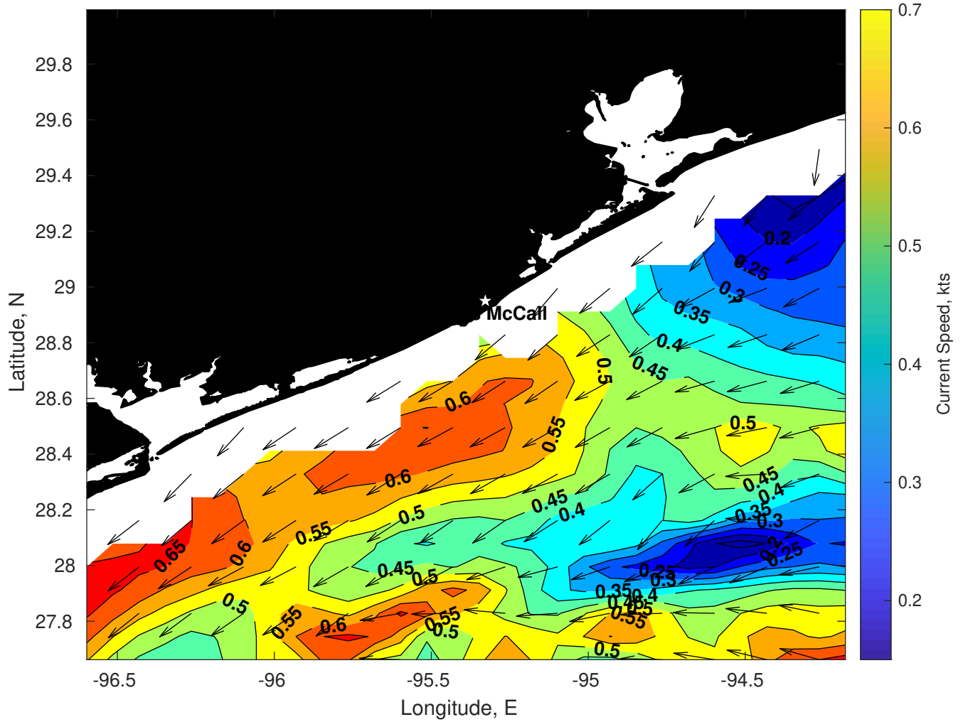
Surface Currents for Brooks McCall at 23-Feb-2026 00:00:00
