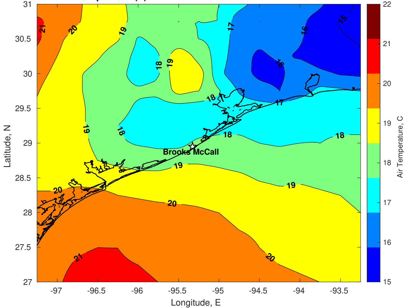
Air Temperature (C) for Brooks McCall at 24-Feb-2026
