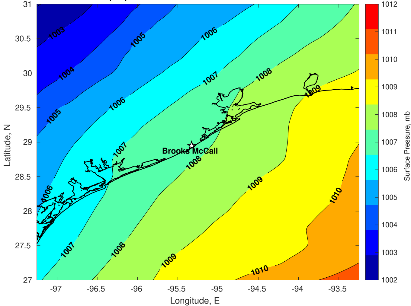
Surface Pressure (mb) for Brooks McCall at 26-Feb-2026 00:00:00
