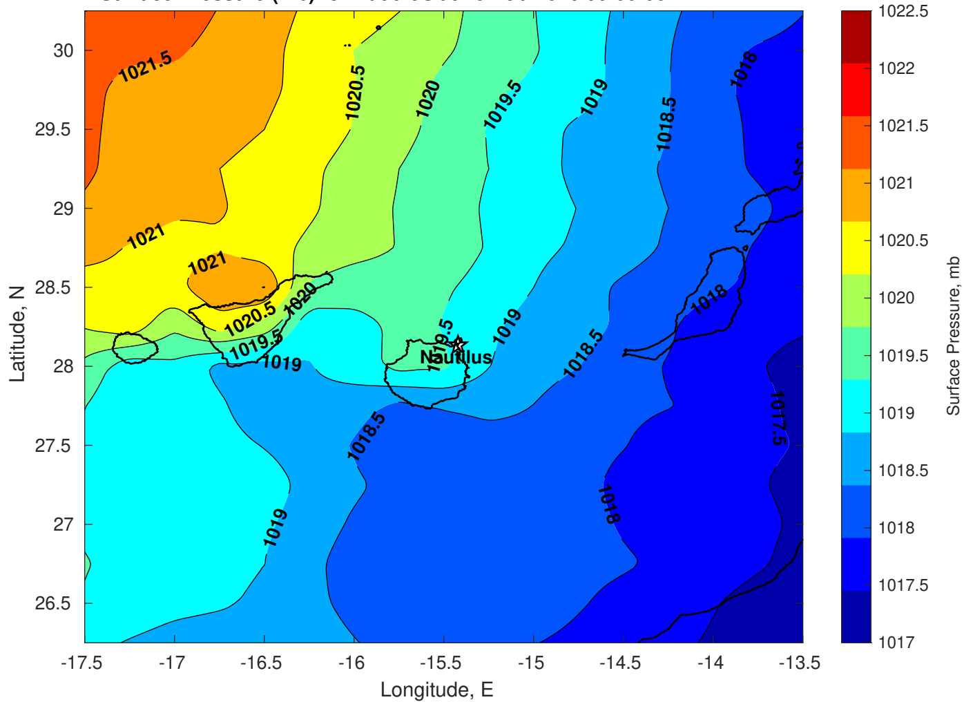
Surface Pressure (mb) for Nautilus at 26-Feb-2026 00:00:00
