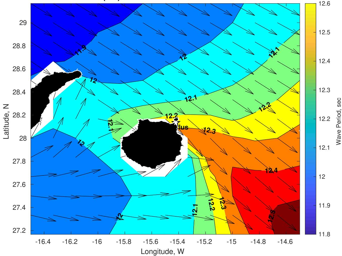
GFS Wave Period (sec) for Nautilus at 24-Feb-2026 09:00:00
