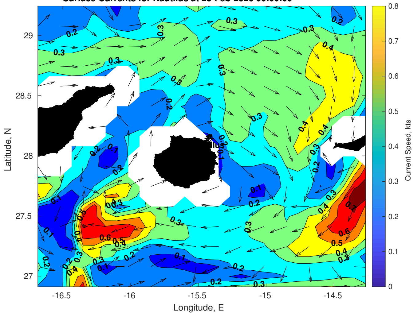
Surface Currents for Nautilus at 23-Feb-2026 00:00:00
