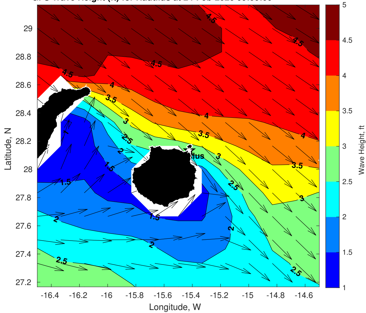
GFS Wave Height (ft) for Nautilus at 24-Feb-2026 09:00:00
