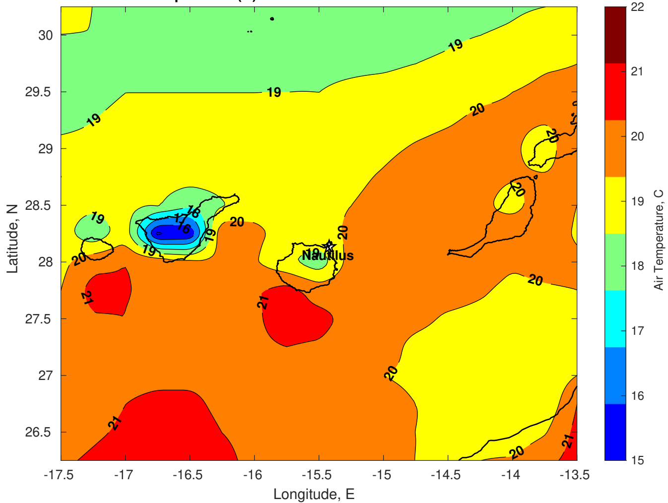
Air Temperature (C) for Nautilus at 24-Feb-2026
