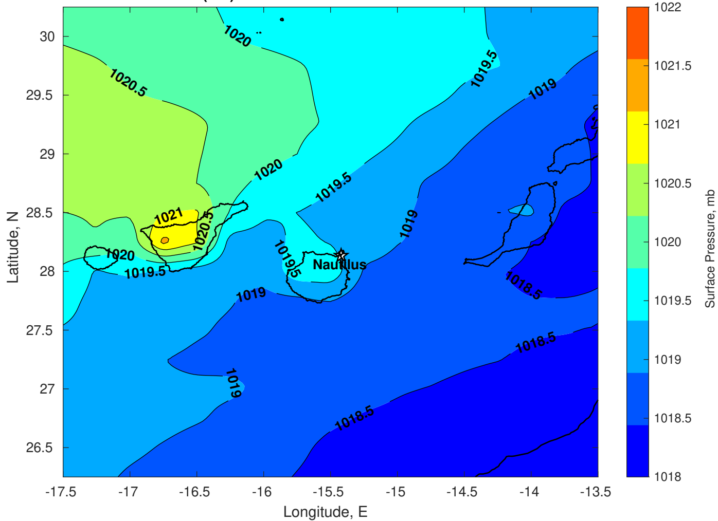
Surface Pressure (mb) for Nautilus at 25-Feb-2026 00:00:00
