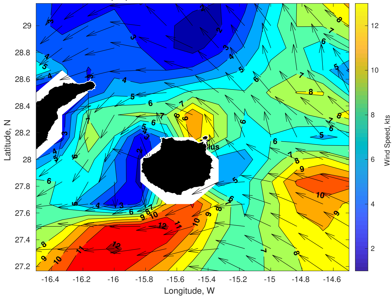
GFS Winds (kts) for Nautilus at 24-Feb-2026 09:00:00
