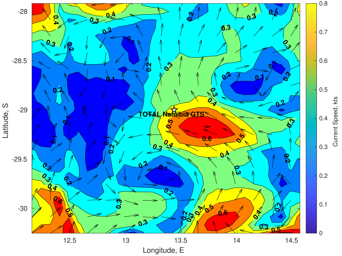
Surface Currents for TOTAL Namibia GTS at 13-Jul-2025 00:00:00
