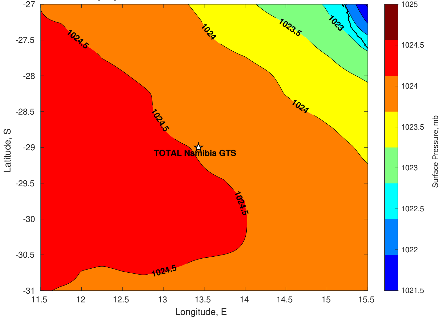
Surface Pressure (mb) for TOTAL Namibia GTS at 05-Oct-2025 09:00:00
