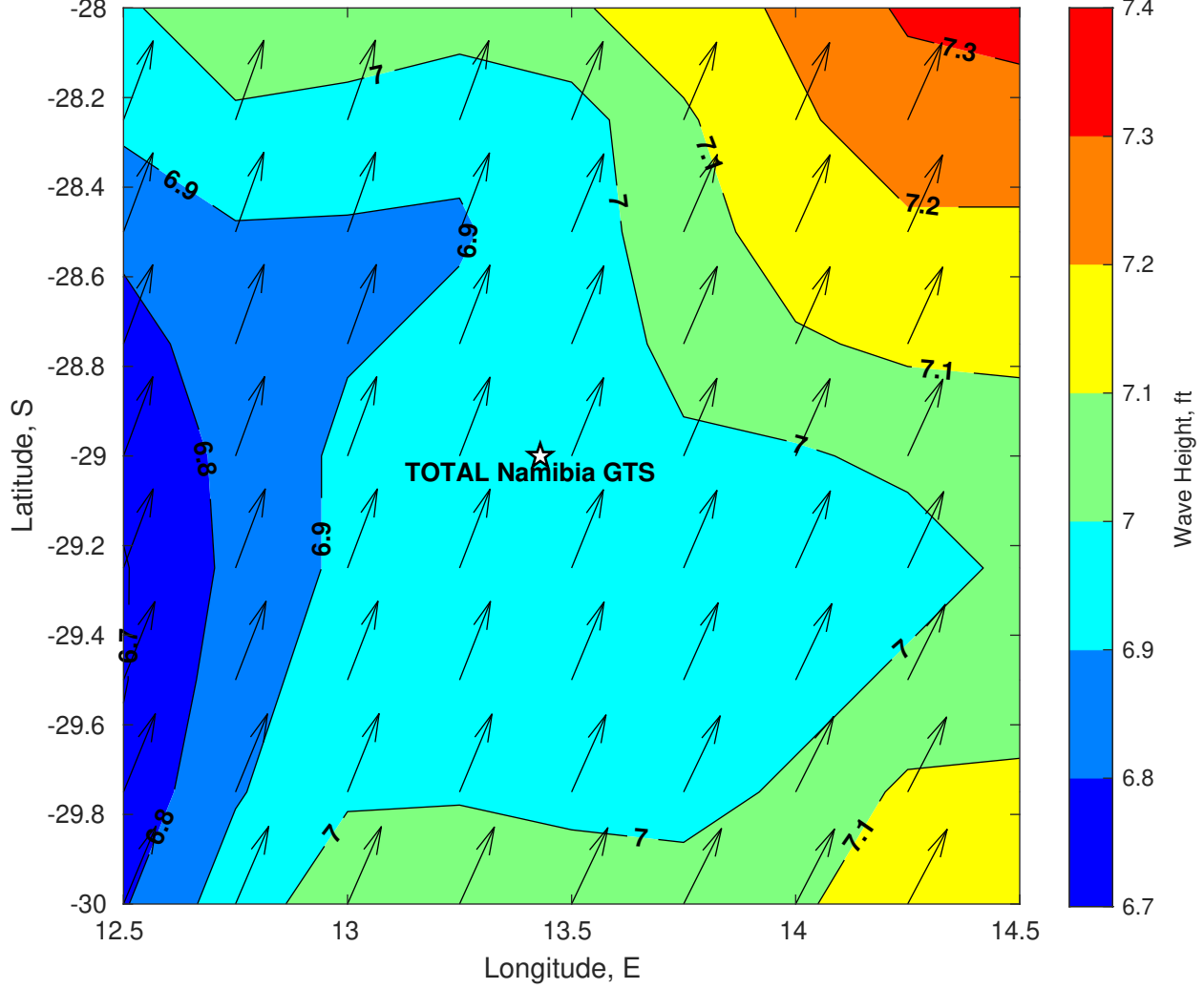
Wave Height (ft) for TOTAL Namibia GTS at 13-Jul-2025 21:00:00
