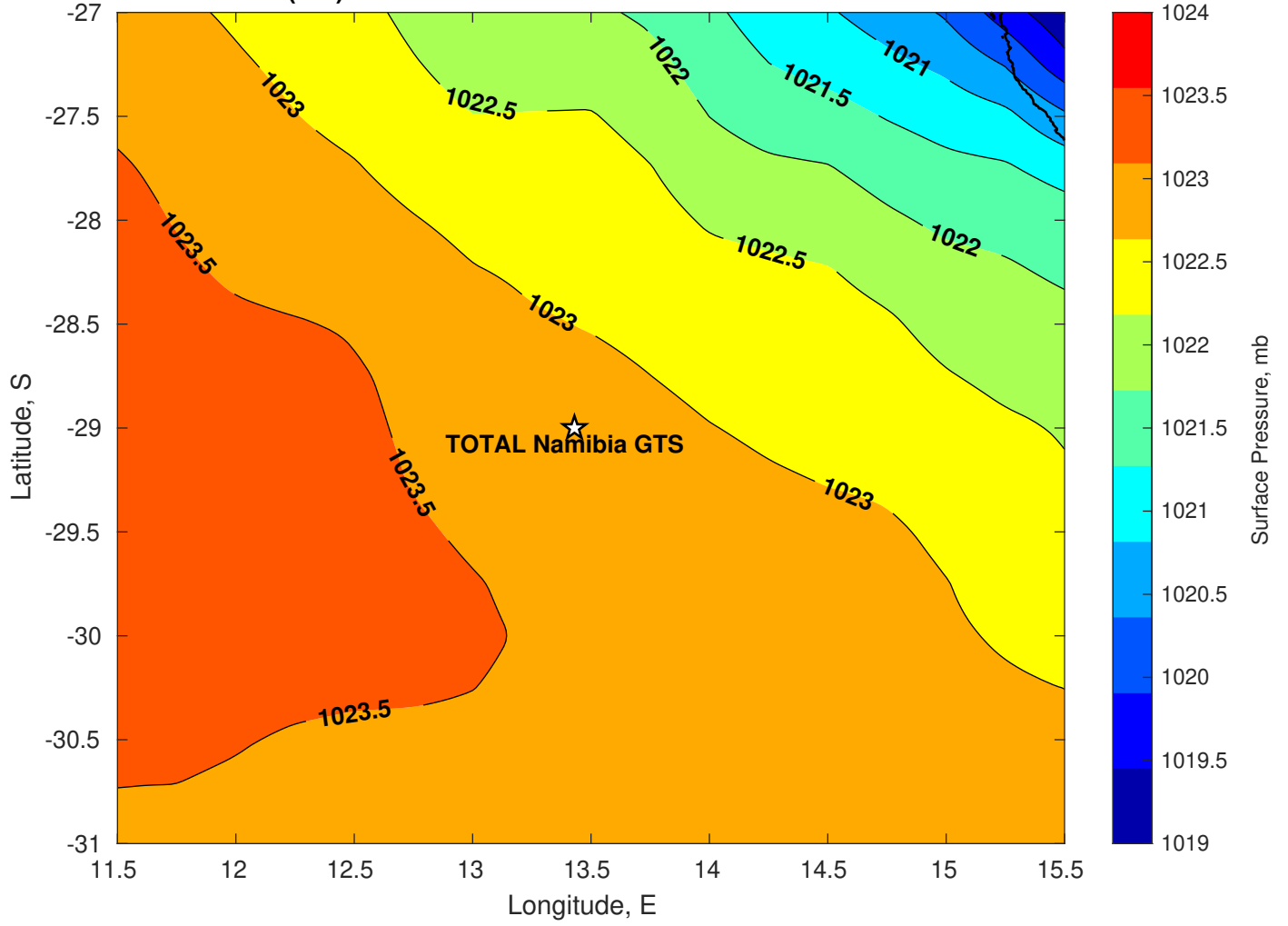
Surface Pressure (mb) for TOTAL Namibia GTS at 15-Jul-2025 12:00:00
