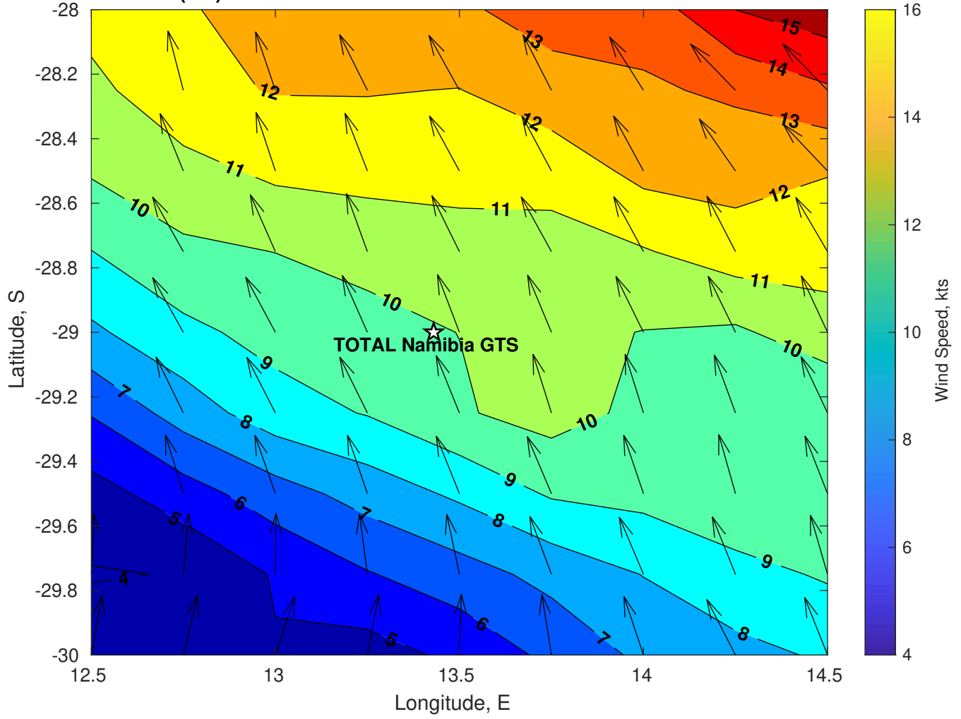
Winds (kts) for TOTAL Namibia GTS at 13-Jul-2025 21:00:00
