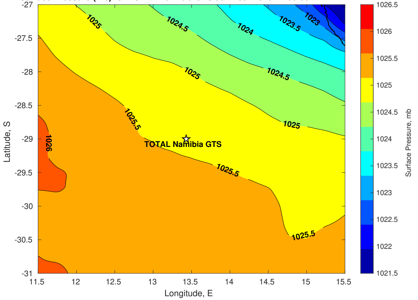
Surface Pressure (mb) for TOTAL Namibia GTS at 14-Jul-2025 12:00:00
