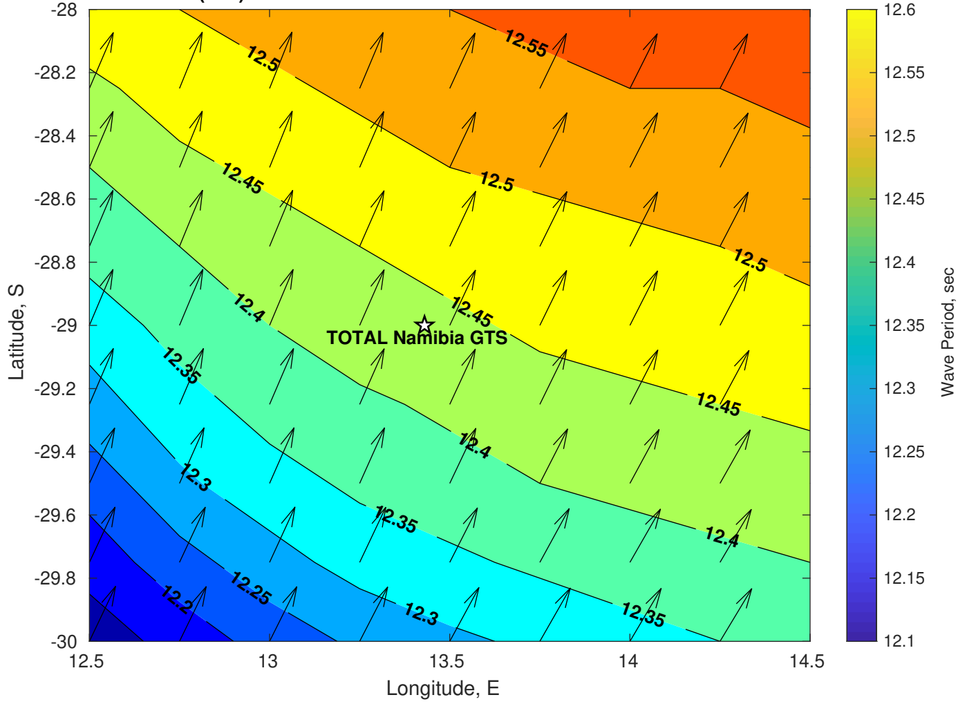
Wave Period (sec) for TOTAL Namibia GTS at 13-Jul-2025 21:00:00
