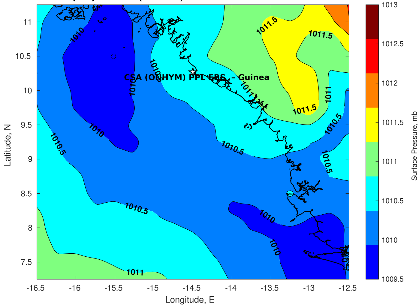
Surface Pressure (mb) for CSA (ONHYM) PPL EBS - Guinea at 26-Feb-2026 00:00:00
