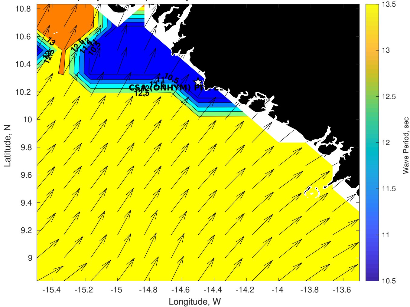
GFS Wave Period (sec) for CSA (ONHYM) PPL EBS - Guinea at 24-Feb-2026 09:00:00
