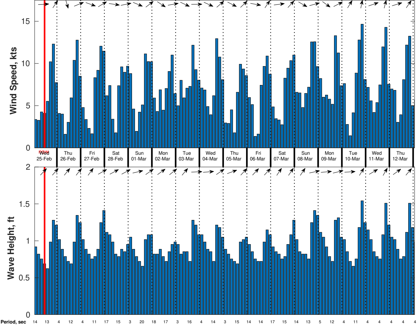
Wind & Wave Forecast for CSA (ONHYM) PPL EBS - Guinea from 24-Feb-2026 01:00:00 to 12-Mar-2026 01:00:00
