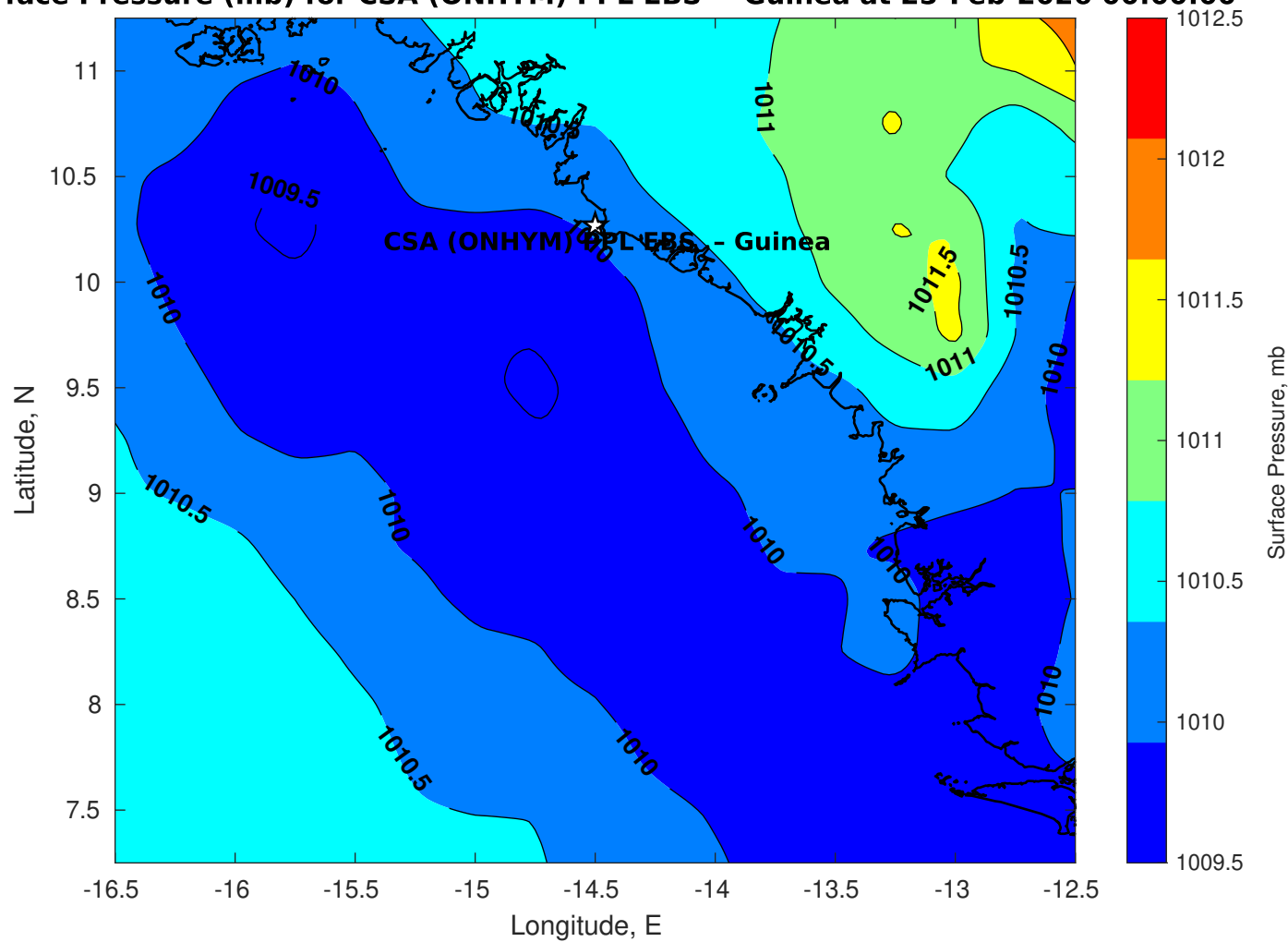
Surface Pressure (mb) for CSA (ONHYM) PPL EBS - Guinea at 25-Feb-2026 00:00:00
