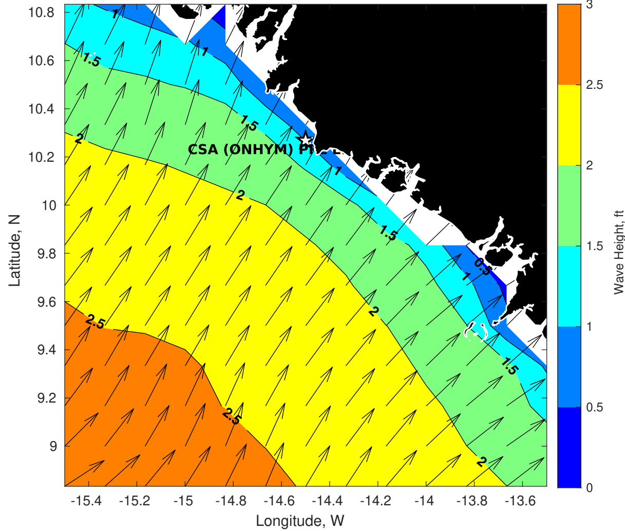
GFS Wave Height (ft) for CSA (ONHYM) PPL EBS - Guinea at 24-Feb-2026 09:00:00
