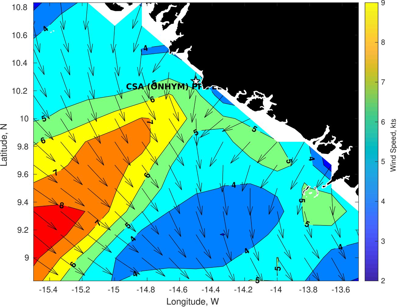
GFS Winds (kts) for CSA (ONHYM) PPL EBS - Guinea at 24-Feb-2026 09:00:00
