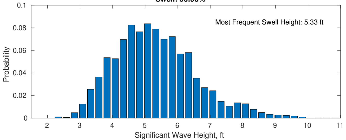
Swell: 99.93%
