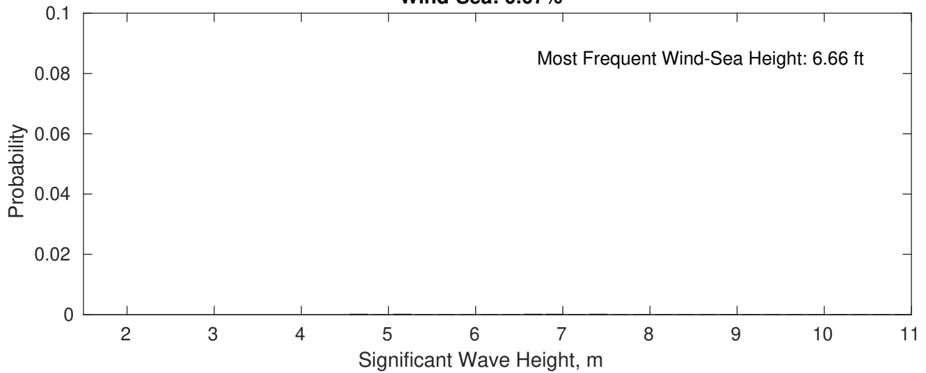
Wind-Sea: 0.07%
