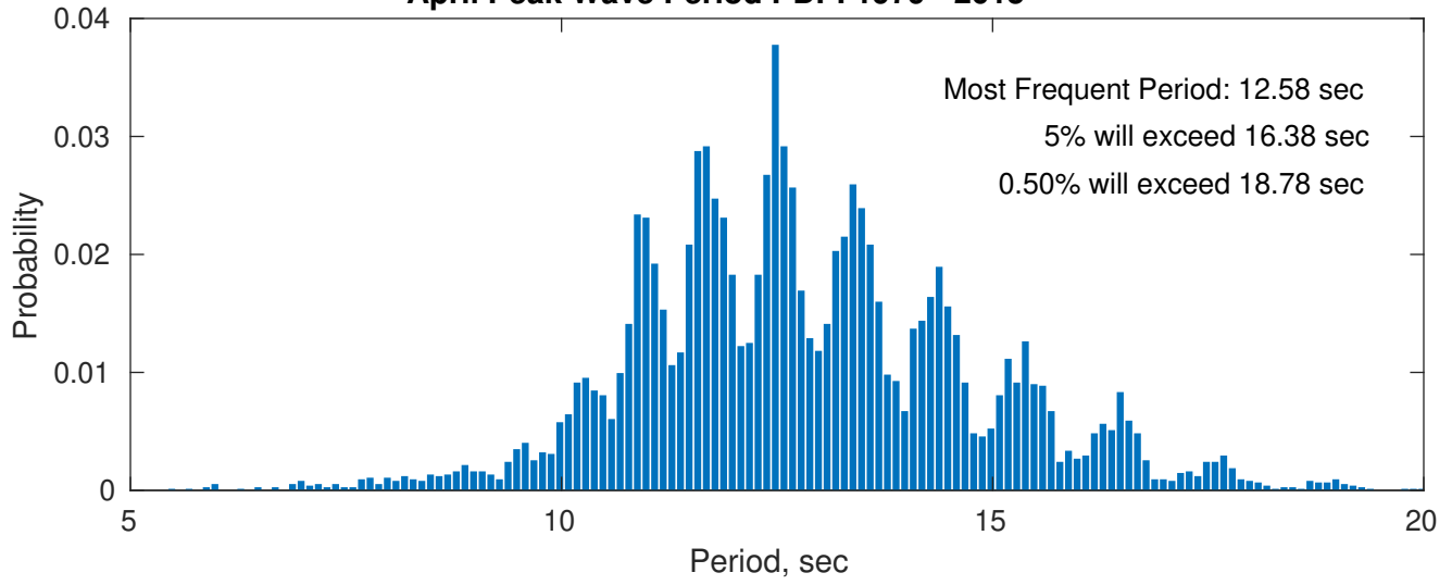
Wind-Sea: 0.07%
