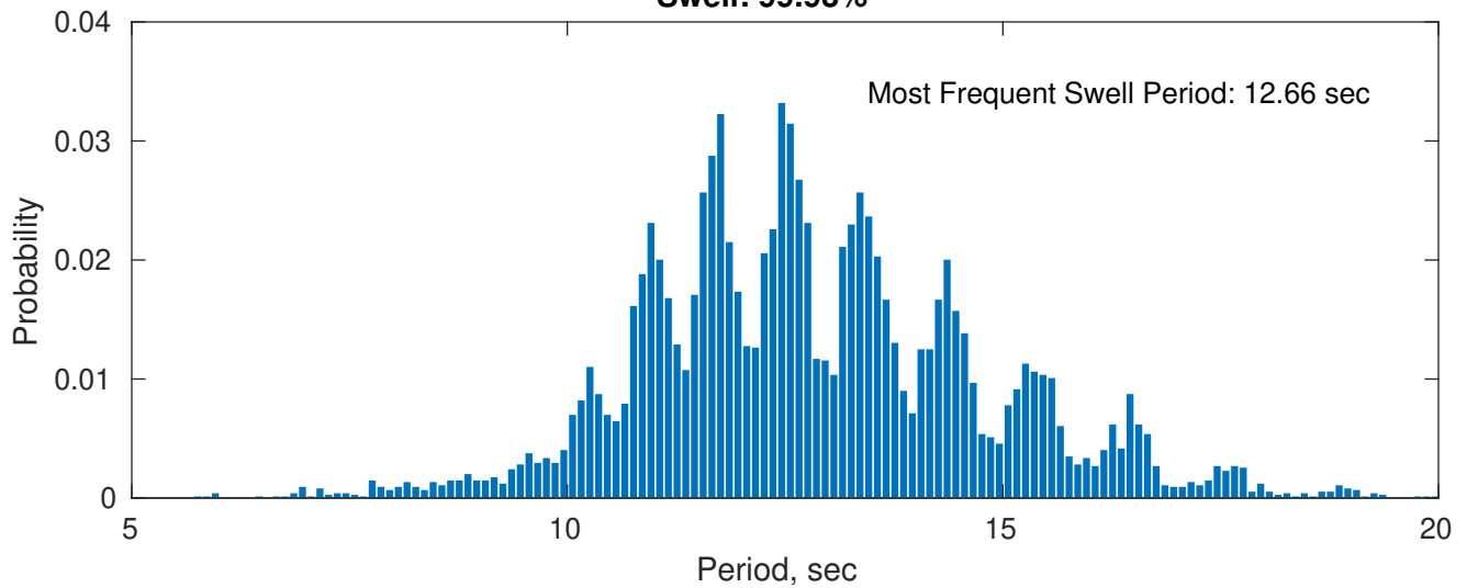
Swell: 99.93%
