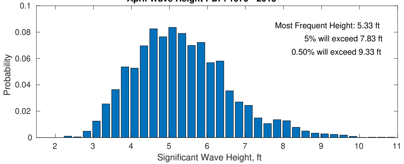
Wind-Sea: 0.07%
