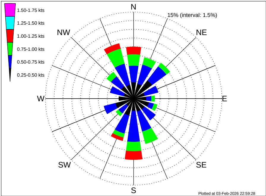
Angola Namibia CRS Luanda (BU-LU) Climatological Surface Current Rose for August: 1995 - 2012
