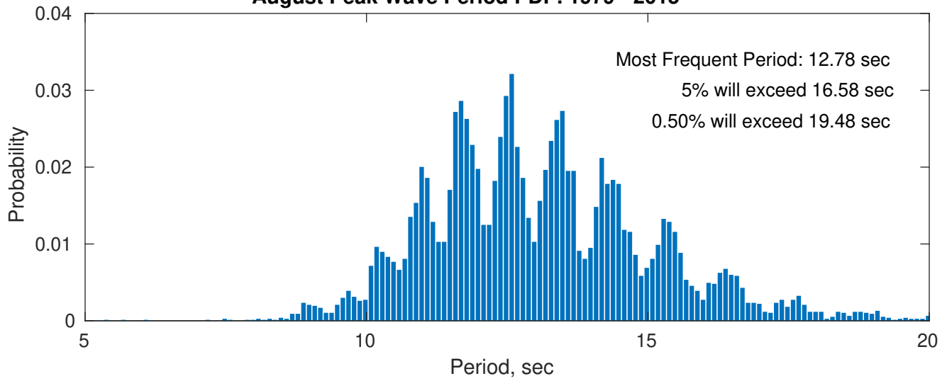
Wind-Sea: 0.01%
