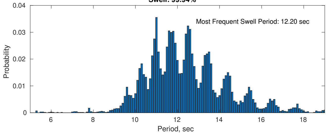
Swell: 99.94%
