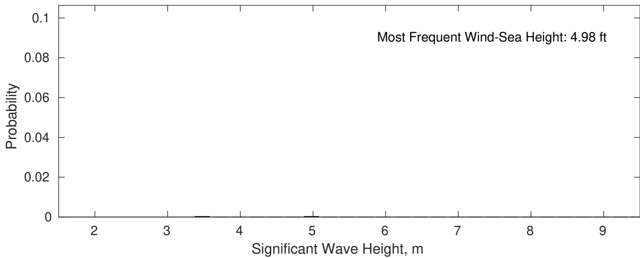
Wind-Sea: 0.06%
