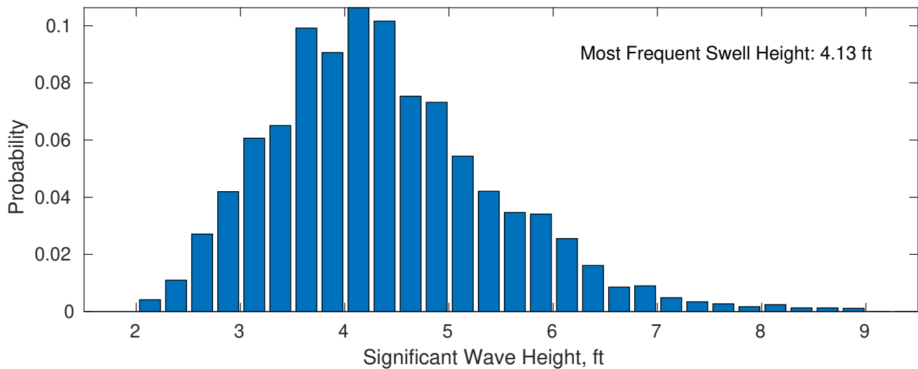
Swell: 99.94%
