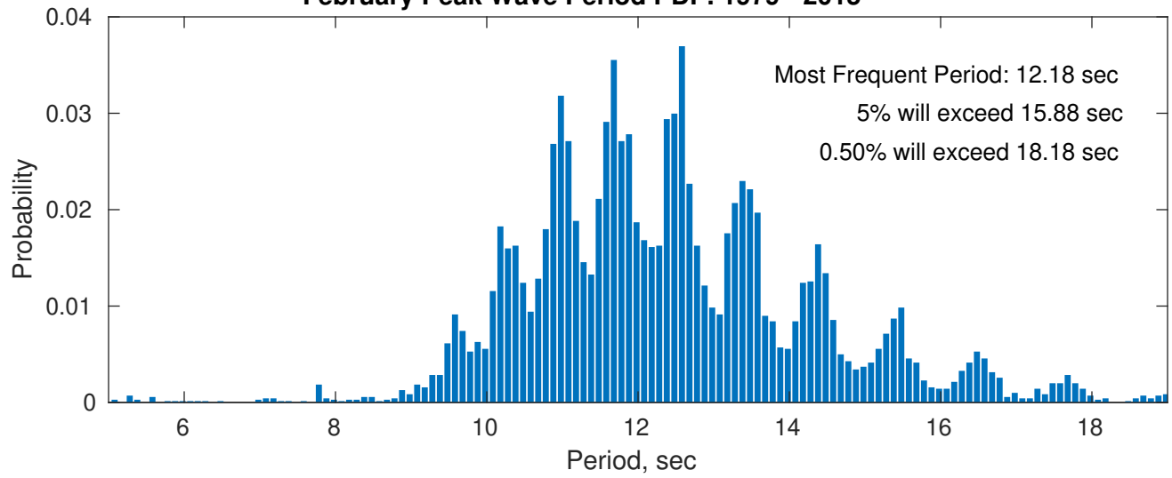
Wind-Sea: 0.06%
