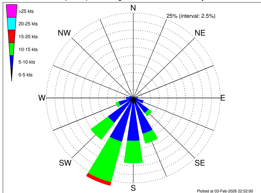
Angola Namibia CRS Luanda (BU-LU) Climatological Wind Rose for February: 1979 - 2015
