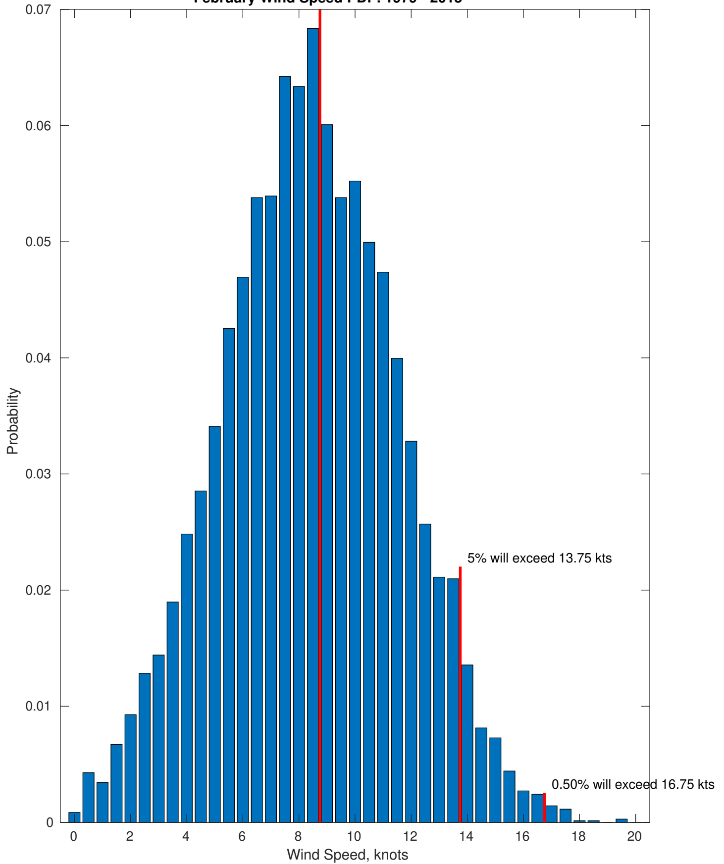
Most Frequent Wind Speed: 8.75 kts February Wind Speed PDF: 1979 - 2015
