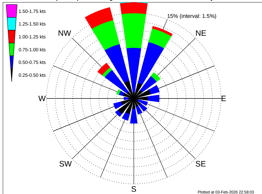
Angola Namibia CRS Luanda (BU-LU) Climatological Surface Current Rose for July: 1995 - 2012
