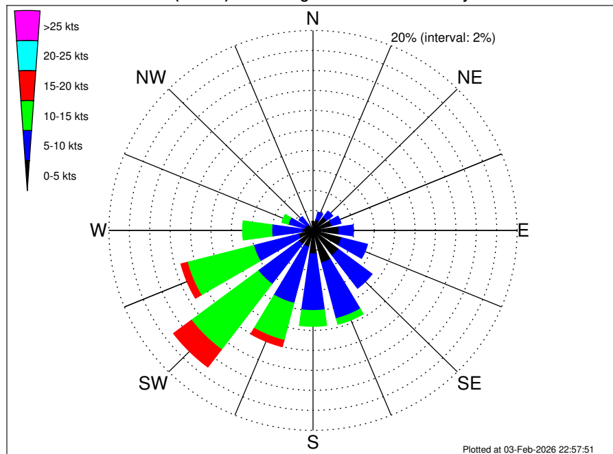
Angola Namibia CRS Luanda (BU-LU) Climatological Wind Rose for July: 1979 - 2015
