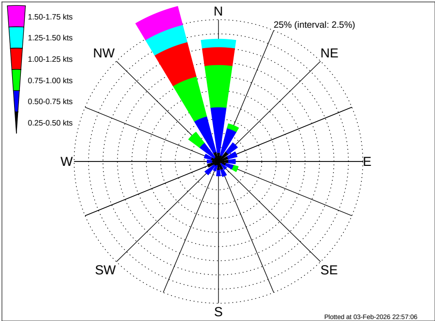
Angola Namibia CRS Luanda (BU-LU) Climatological Surface Current Rose for June: 1995 - 2012
