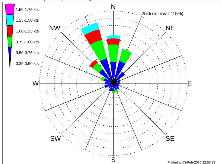
Angola Namibia CRS Luanda (BU-LU) Climatological Surface Current Rose for March: 1995 - 2012
