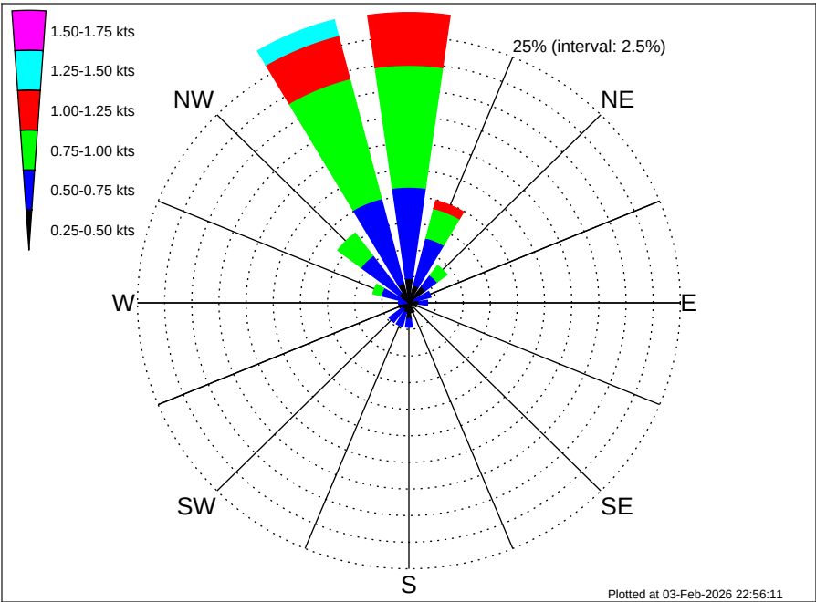
Angola Namibia CRS Luanda (BU-LU) Climatological Surface Current Rose for May: 1995 - 2012
