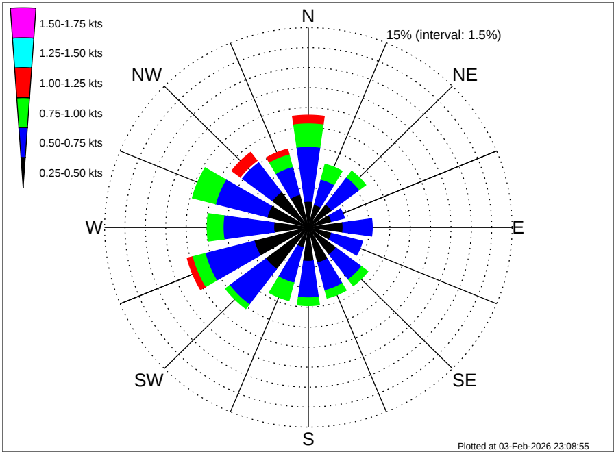
Angola Namibia CRS Mocamedes (BU-MO) Climatological Surface Current Rose for April: 1995 - 2012
