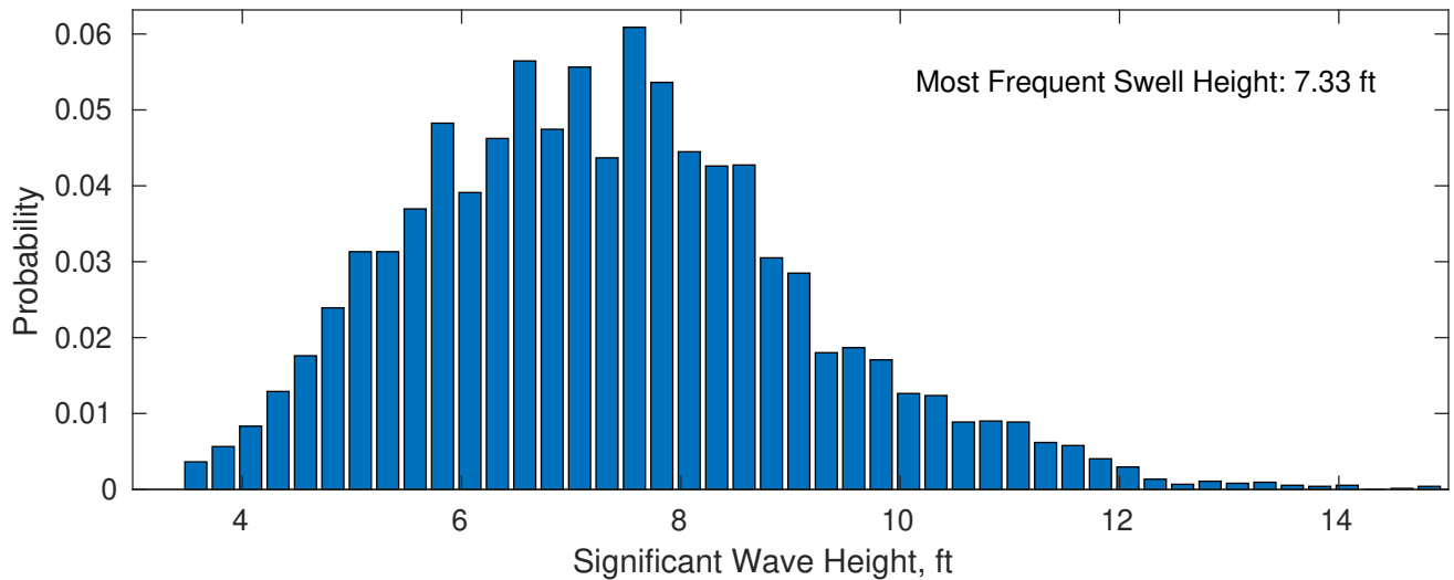
Swell: 94.31%
