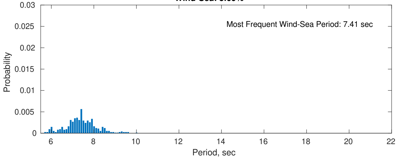
Wind-Sea: 5.69%
