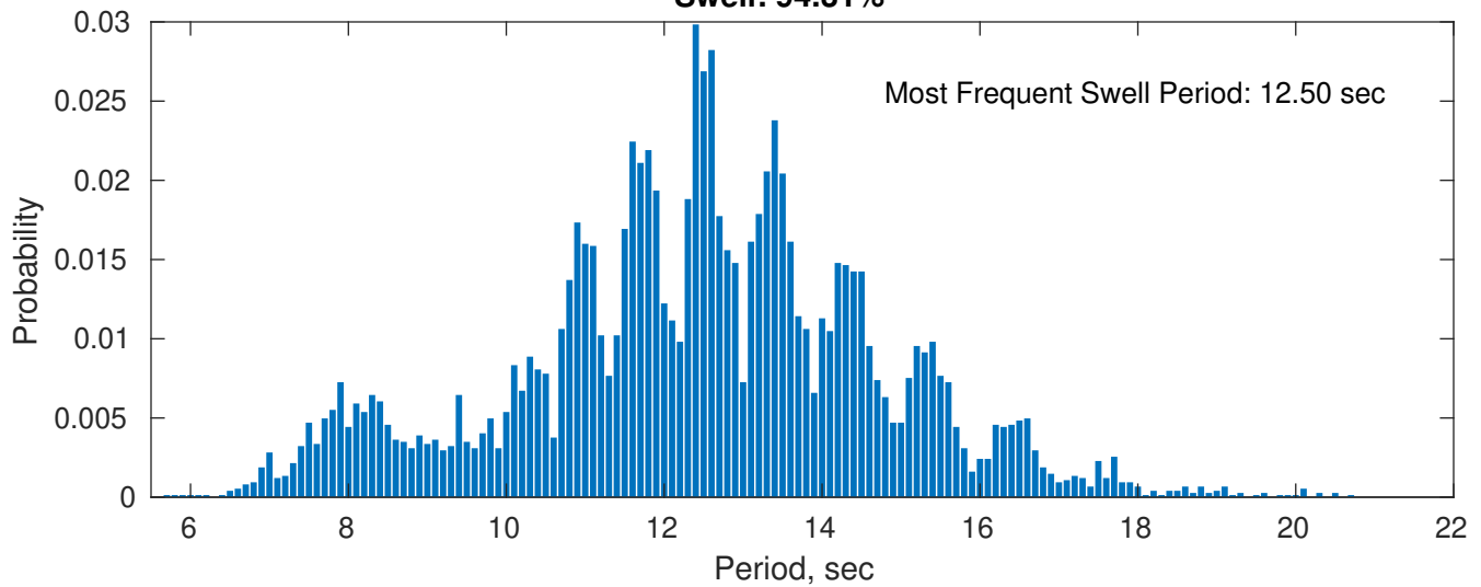
Swell: 94.31%
