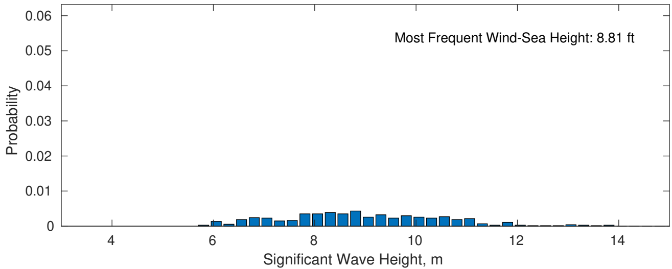
Wind-Sea: 5.69%
