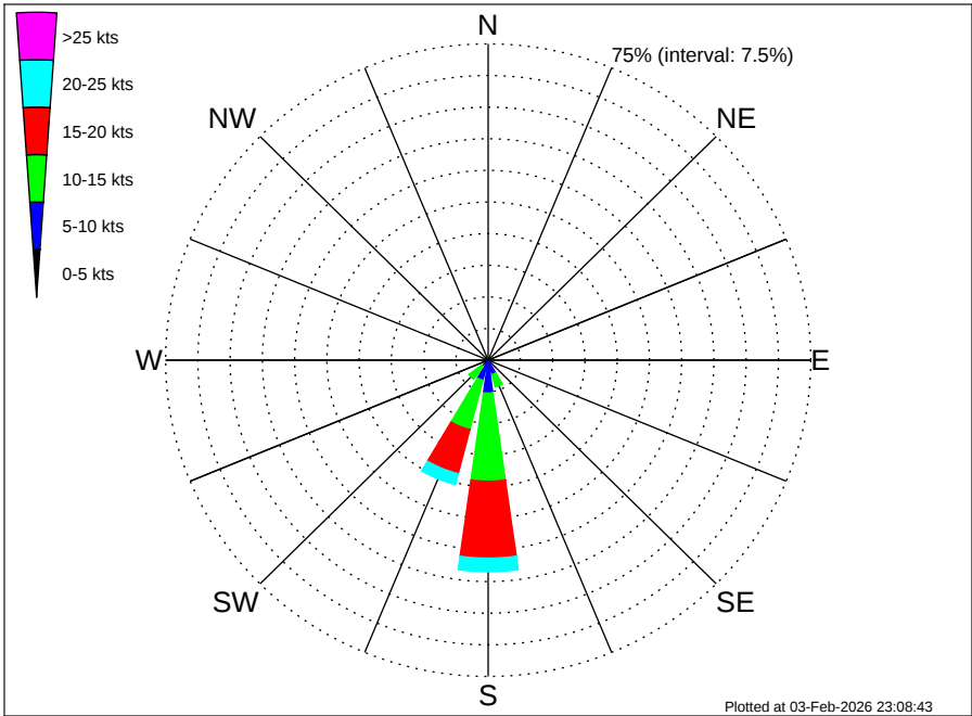
Angola Namibia CRS Mocamedes (BU-MO) Climatological Wind Rose for April: 1979 - 2015
