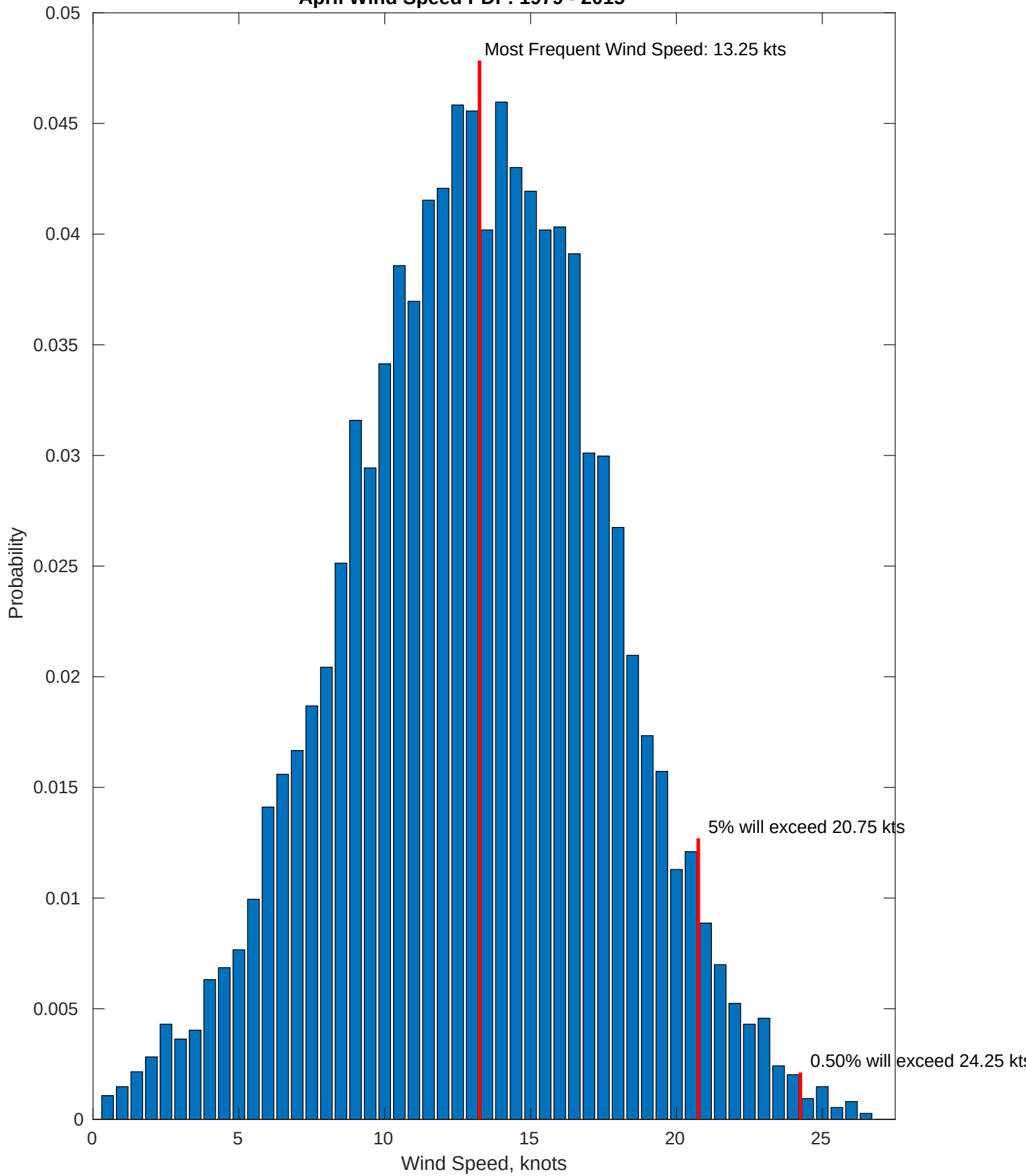
April Wind Speed PDF: 1979 - 2015
