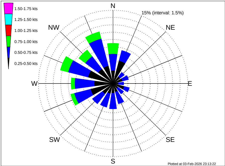
Angola Namibia CRS Mocamedes (BU-MO) Climatological Surface Current Rose for August: 1995 - 2012
