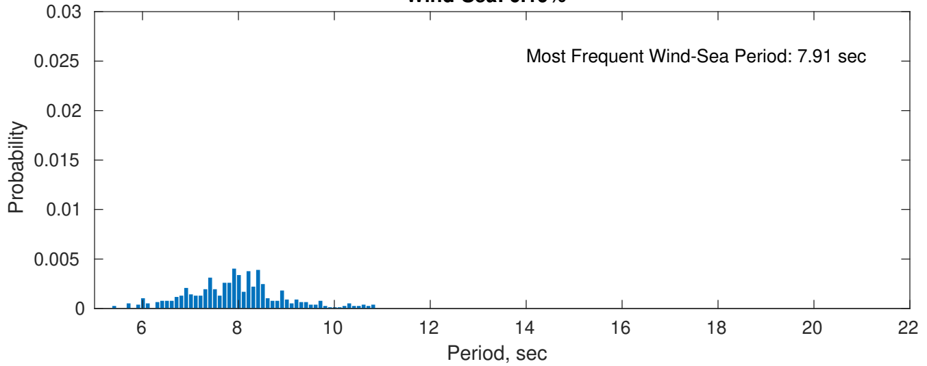
Wind-Sea: 6.19%
