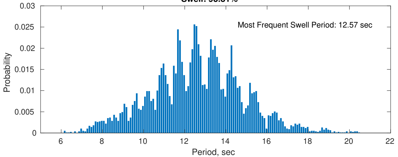
Swell: 93.81%
