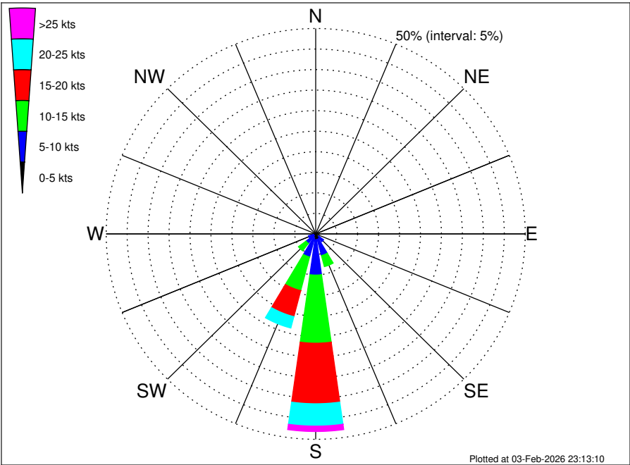
Angola Namibia CRS Mocamedes (BU-MO) Climatological Wind Rose for August: 1979 - 2015
