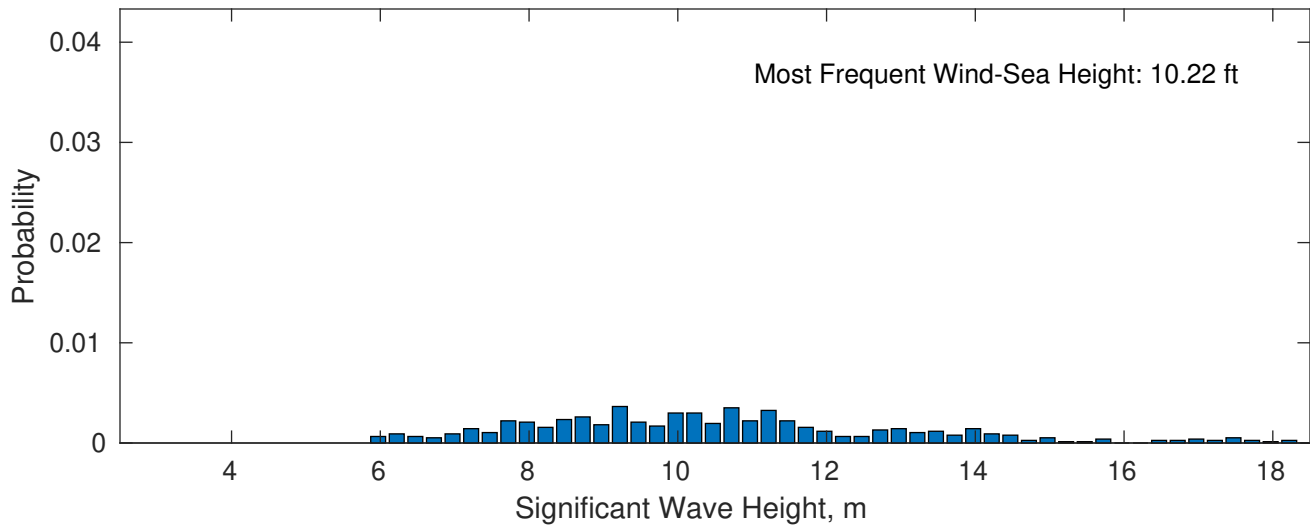
Wind-Sea: 6.19%
