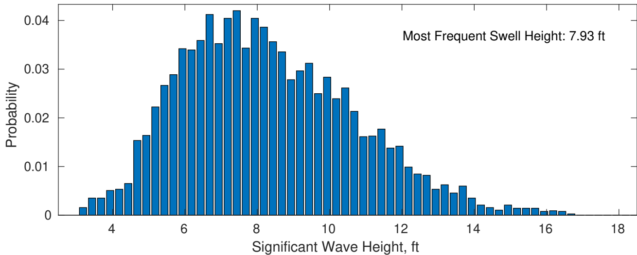
Swell: 93.81%
