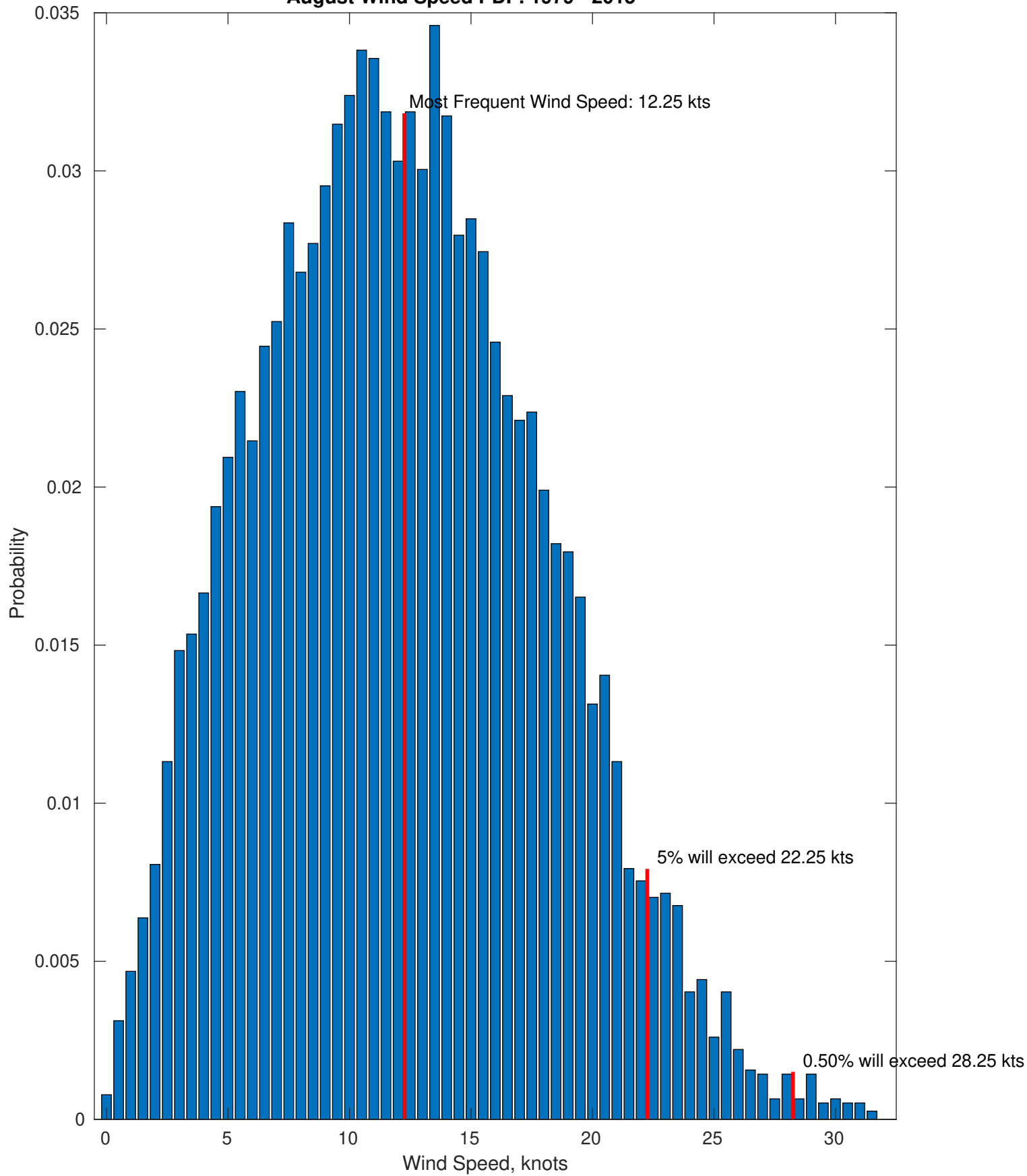
August Wind Speed PDF: 1979 - 2015
