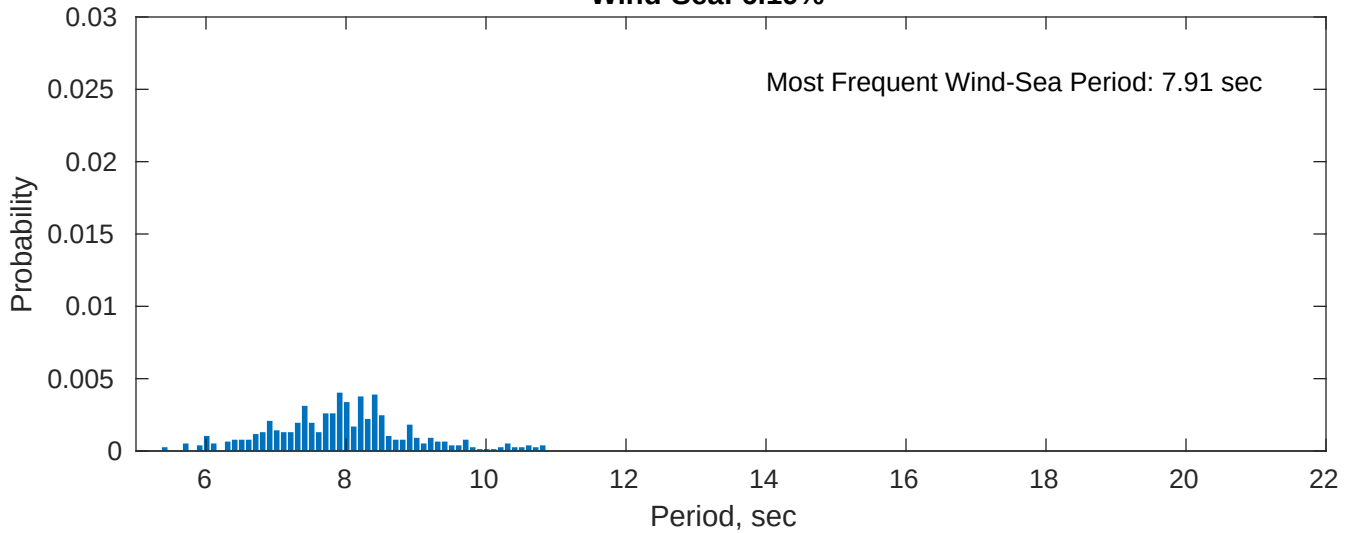
Wind-Sea: 6.19%
