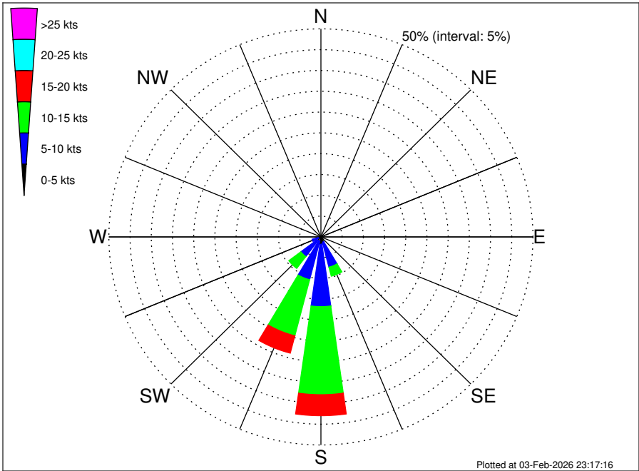
Angola Namibia CRS Mocamedes (BU-MO) Climatological Wind Rose for December: 1979 - 2015
