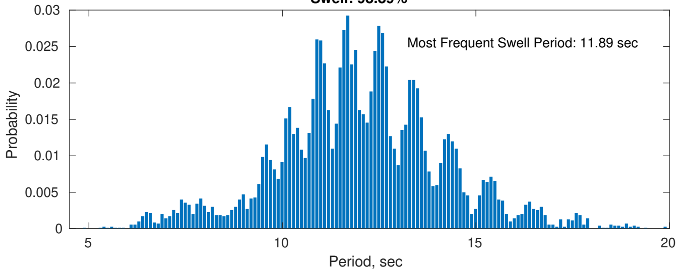
Swell: 98.89%
