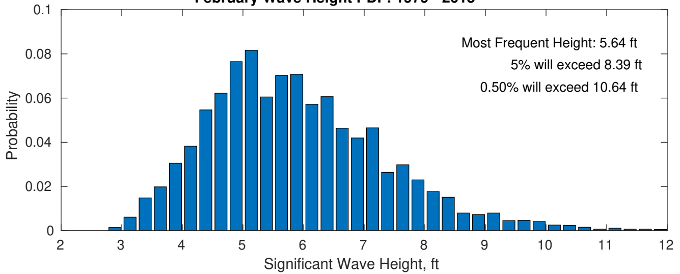
Wind-Sea: 1.11%
