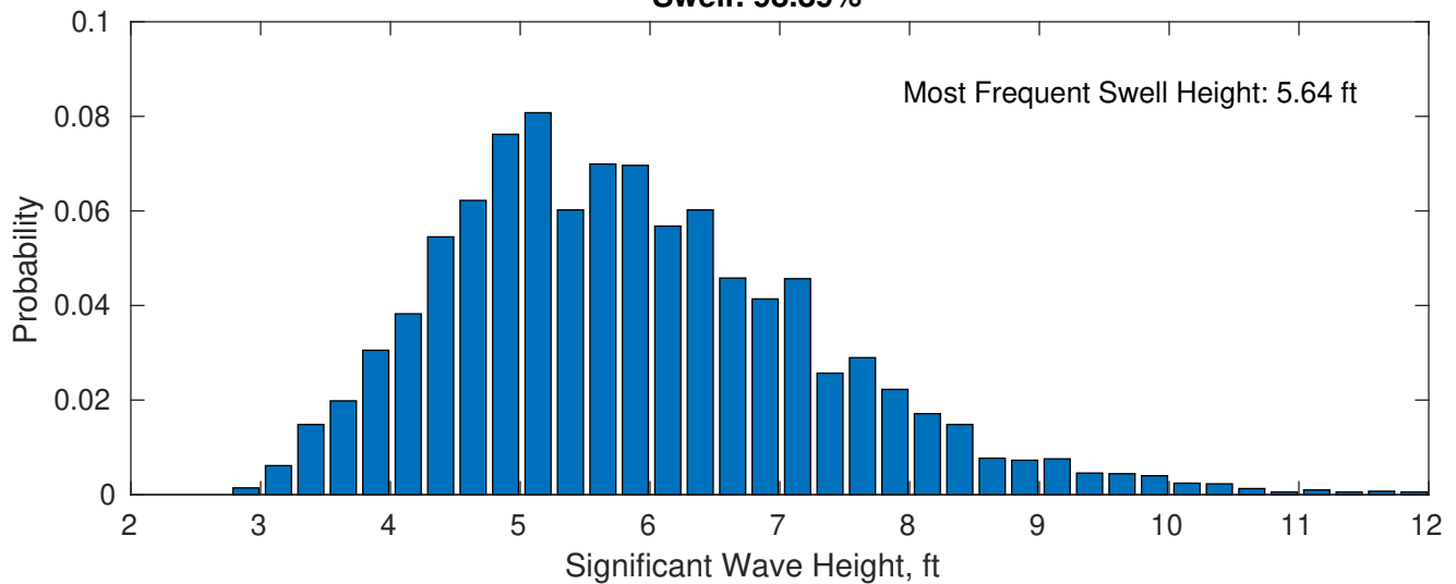
Swell: 98.89%
