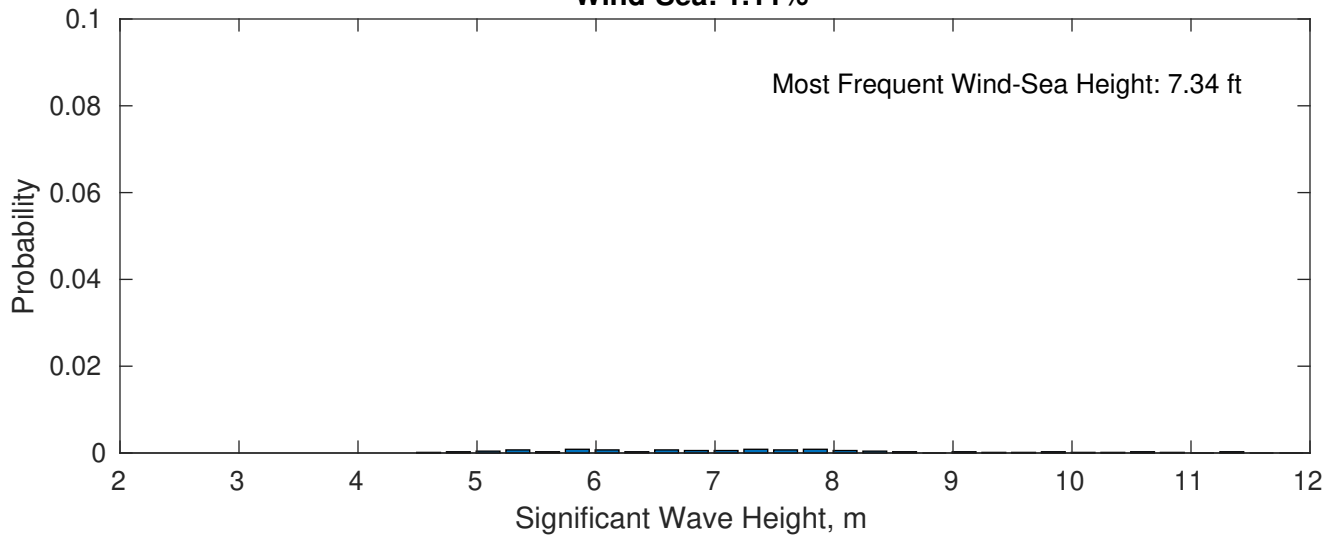
Wind-Sea: 1.11%
