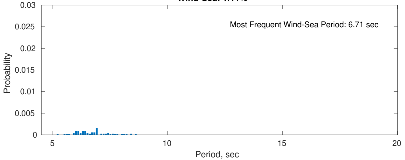
Wind-Sea: 1.11%
