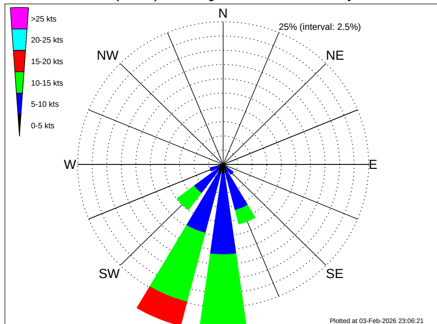
Angola Namibia CRS Mocamedes (BU-MO) Climatological Wind Rose for February: 1979 - 2015
