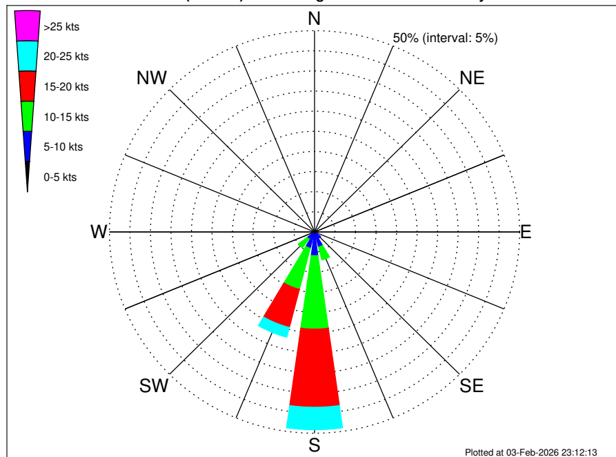
Angola Namibia CRS Mocamedes (BU-MO) Climatological Wind Rose for July: 1979 - 2015
