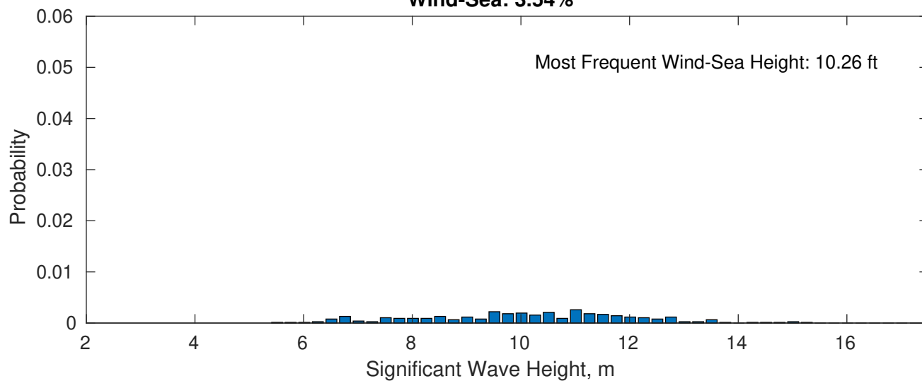
Wind-Sea: 3.54%
