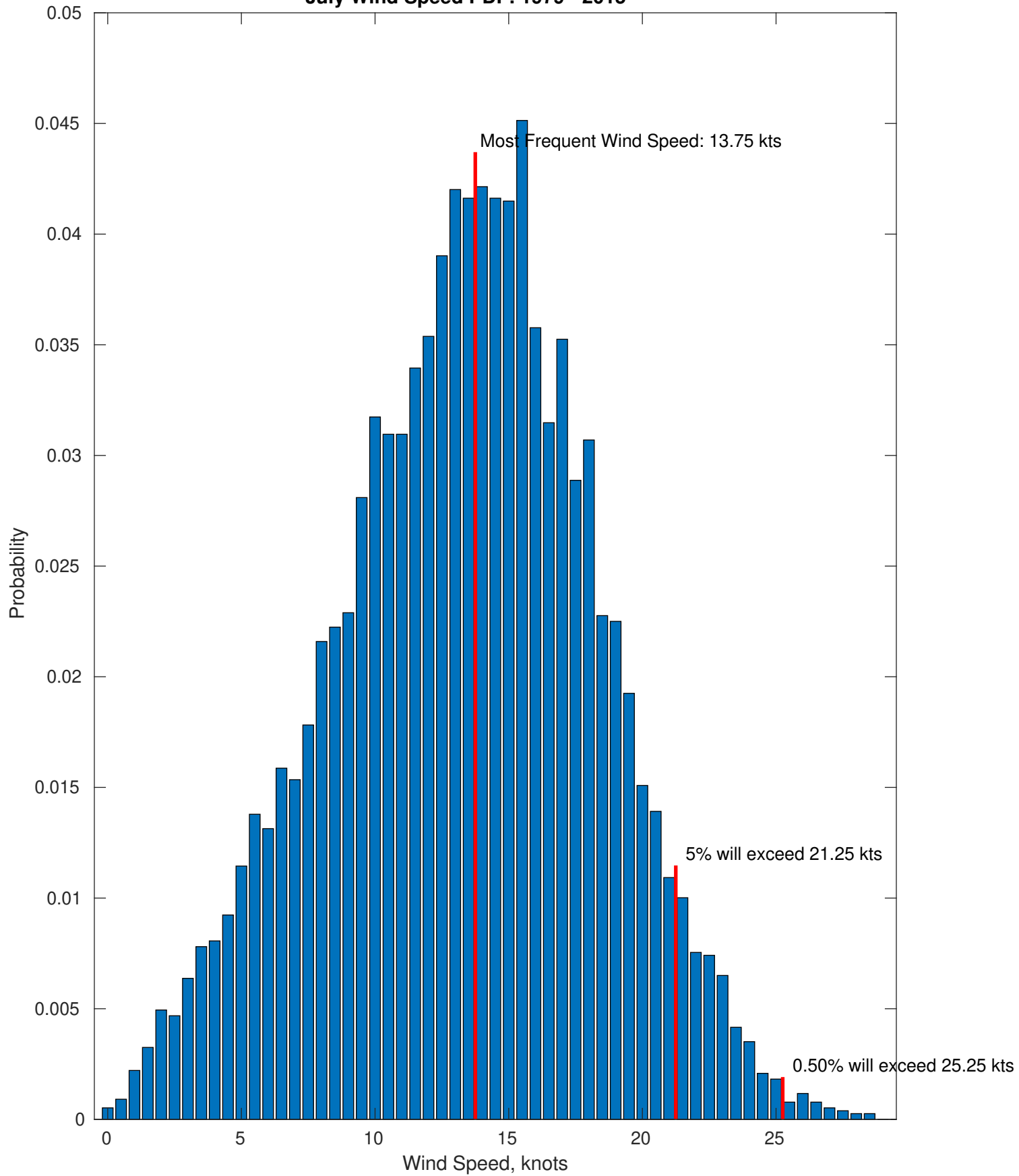
July Wind Speed PDF: 1979 - 2015
