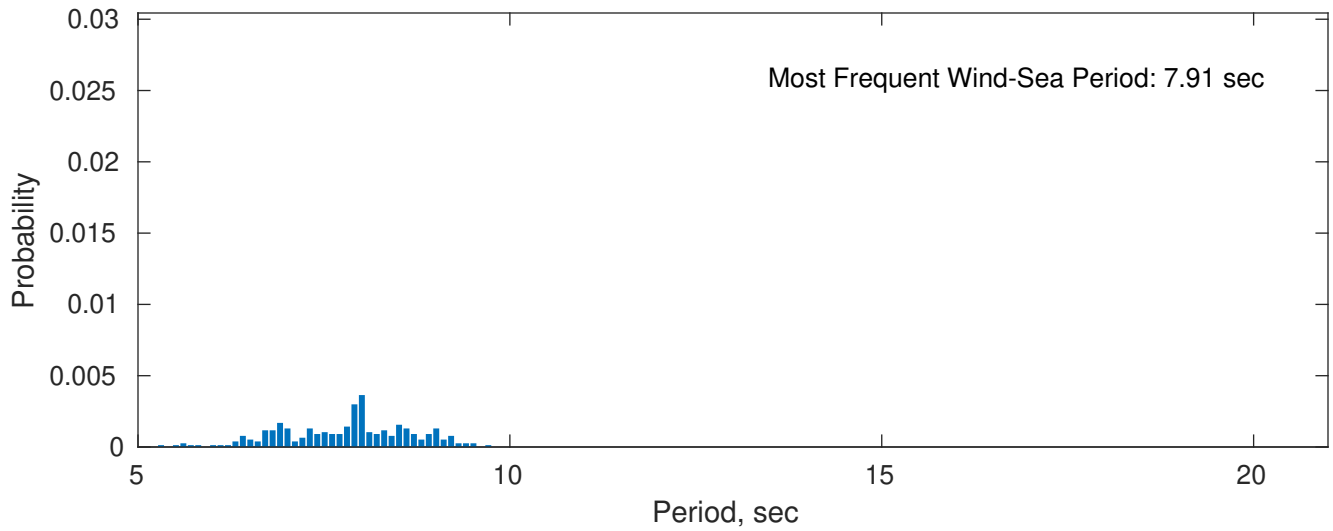
Wind-Sea: 3.54%
