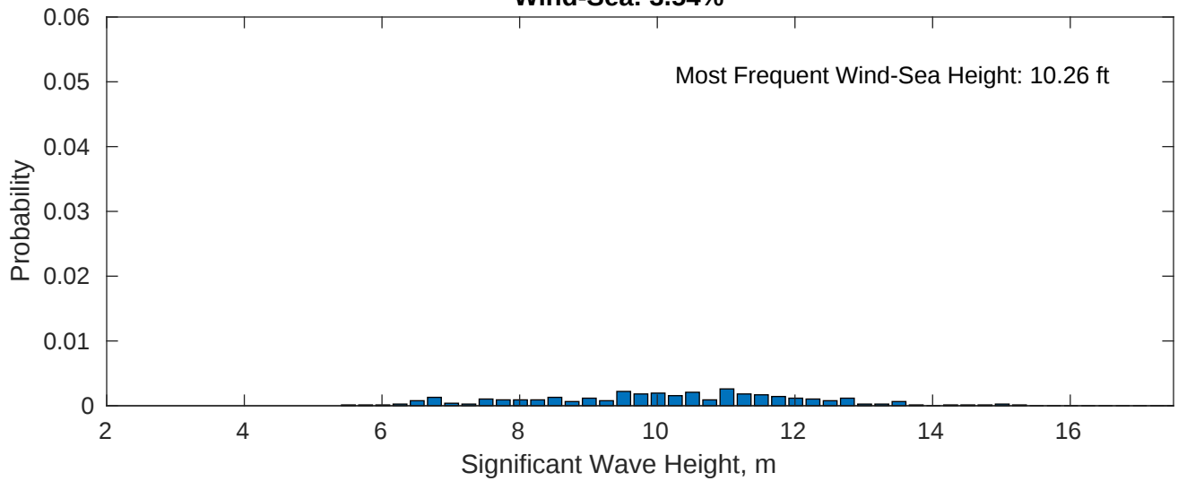
Wind-Sea: 3.54%
