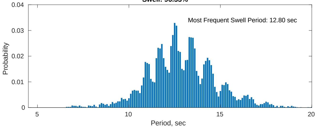
Swell: 96.33%
