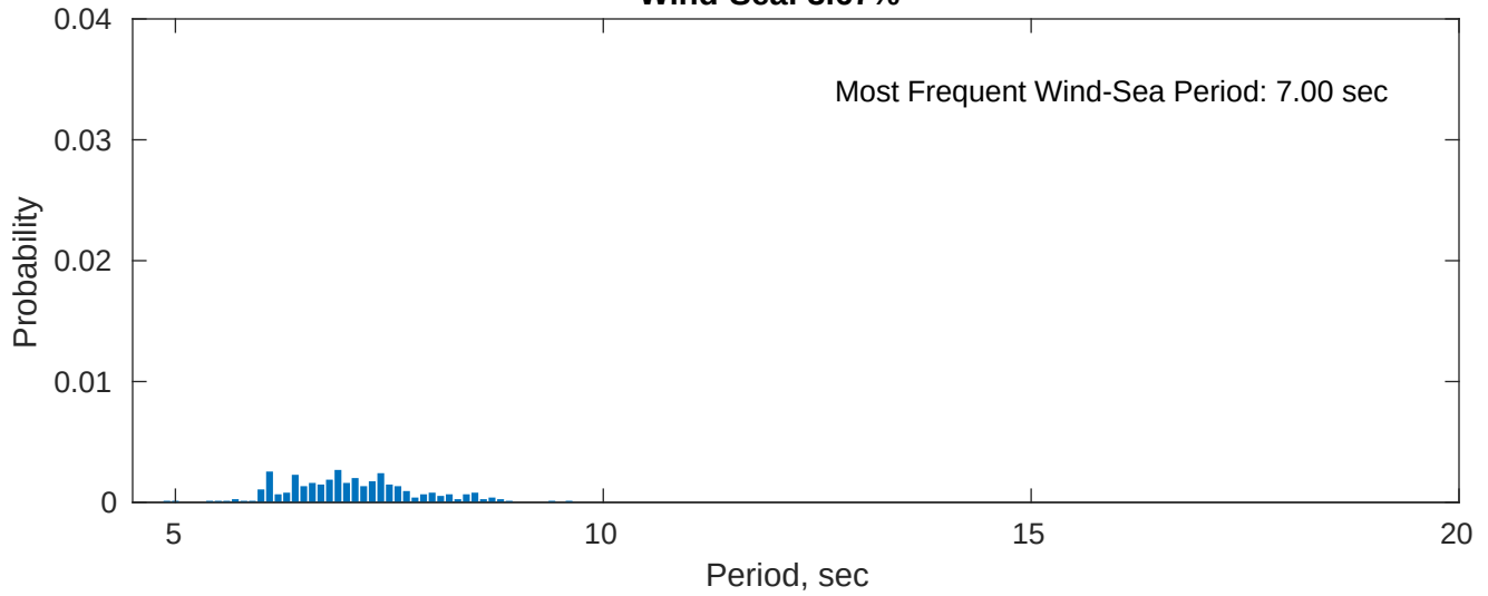
Wind-Sea: 3.67%
