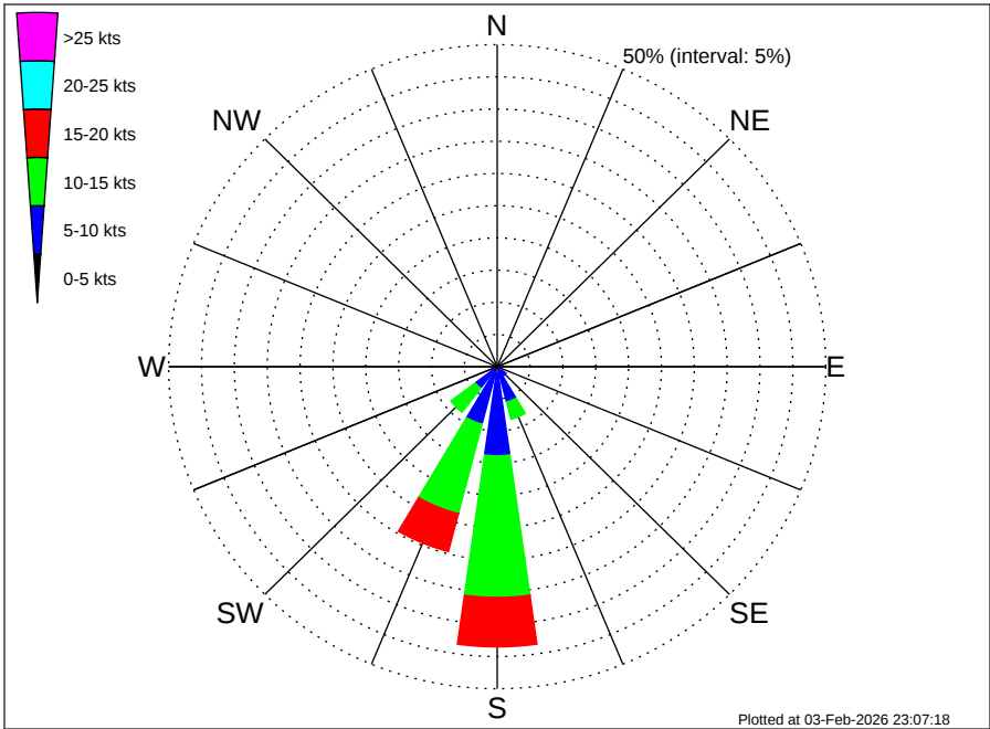
Angola Namibia CRS Mocamedes (BU-MO) Climatological Wind Rose for March: 1979 - 2015
